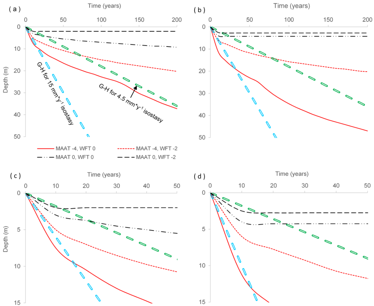
425 Figure 7. Early and mid-Holocene freezing depth in the first 50 and 200 years with MAAT -4^{\circ}\text{C} and 0^{\circ}\text{C} ; WFT of 0 and -2^{\circ}\text{C} . (a) 100% freezing, (b) 25% freezing. Also shown are curves of two scenarios of corresponding depths of the fresh-saline water interface, using a 1:40 Ghyben-Hertzberg (G-H) approximation for isostasy of 4.5 and 15\text{ mm y}^{-1} . See text for more details. (c) and (d) are zoomed in of (a) and (b) for the first 50 years. The fast deepening in figures a, and b is due to change in porosity as the freezing front reaches the bedrock (25 m). The legend is the same for all figures.
