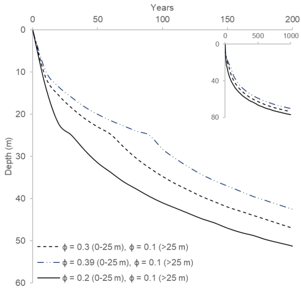
Figure 11. Simulations as in Fig. 9 (MAAT= -4°C, WFT= 0°C), but with 25% freezing.
