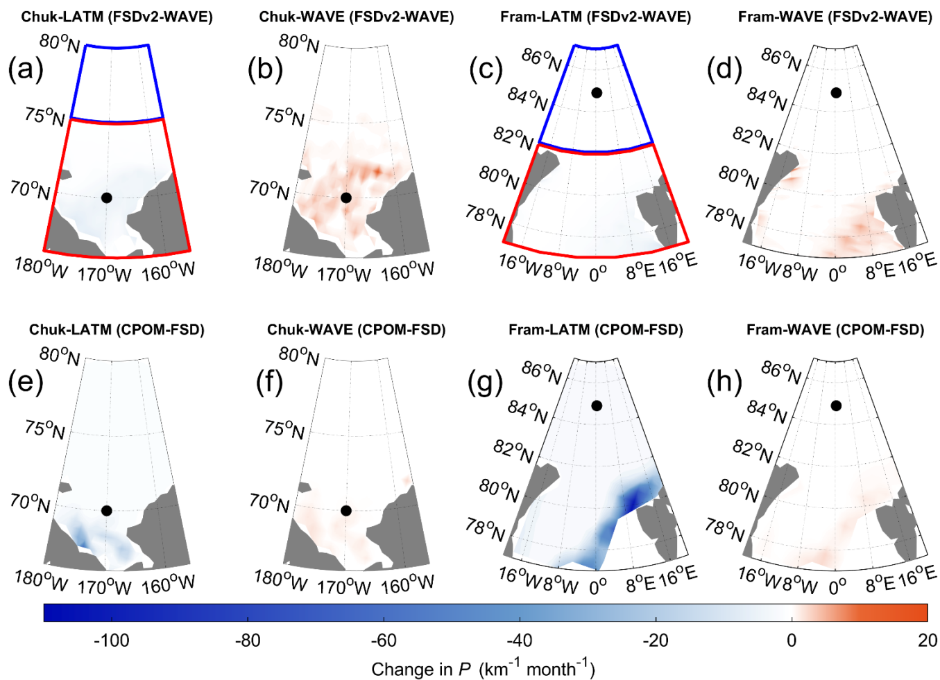
690 Figure 6: Monthly changes of P simulated by the two prognostic models over the period May to July during 2000–2014. (a) Change of FSD arising from lateral melt for FSDv2-WAVE in the Chukchi Sea. (b) is same as (a) but for wave induced P change. (c) and (d) are same as (a) and (b) but in the Fram Strait. (e)–(h) is same as (a)–(d) but for CPOM-FSD. The blue and red box in (a) and (c) show the northern and southern region of the two study regions. Black dots indicate the location of observations in the study regions.
