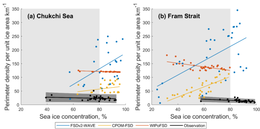
Figure 3: Perimeter density P according to SIC for (a) the Chukchi Sea region and (b) the Fram Strait region. Dark grey shades along the regression lines of the observations mark a 95% confidence interval. The light grey shade marks the MIZ, defined as SIC between 15% and 80%.
