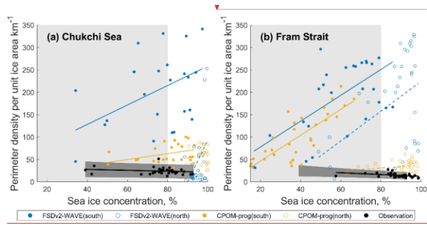
Figure 7: Similar to Figure 3 but show the comparison between observations (black) and two prognostic models (FSDv2-WAVE—blue, CPOM-FSD—yellow) in southern regions (solid circle) and northern regions (hollow circle) of the study region in the Chukchi Sea (a) and the Fram Strait (b).
