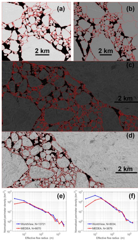
Figure 4: Comparison of perimeter density between (a) WV © image ( \delta = 0.5 m) and (b) MEDEA image ( \delta = 1 m) on 5 June 2013 at 84.9°N, 0.1°E (Fram Strait) is shown in (e) and between (c) WV image ( \delta = 0.5 m) on 1 June 2013 and (d) MEDEA image ( \delta = 1 m) on 31 May 2013 at 70°N, 170°W (Chukchi Sea) is shown in (f). The image size of the co-located scenes shown in (a), (b), (c) and (d) cover an area of 106 km 2 , 82 km 2 , 66 km 2 and 64 km 2 respectively. In panels (e)–(f), N is the number of floes derived from satellite images.
