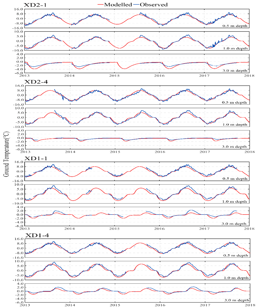
725 Figure A3. Comparison of the simulated (red lines) to observed (blue lines) daily mean ground temperature at 0.5 m, 1.0 m, and 3.0 m depth in four validation boreholes (XD2-1, XD2-4, XD1-1, and XD1-4) during the observation period from 2013 to 2018 (There were some data gaps due to temperature probe failure in some years, at the XD2-1, the data gaps in the record mainly occurred at 0.5-3.0 m in the first half of 2015, at the XD1-1, the data gap in the record at 0.5-3.0 in 2014-2015, at 8-15 m during 2013-2015, at the XD1-4, the data 730 gap in the record in the first half of 2015).
