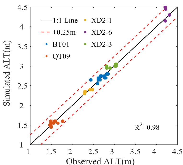
Figure 3. Comparison between annually observed ALT and simulated at different sites (the TB01 and QT09 370 (Liu et al. (2019), Zhao et al. (2021) observed from period 2005 to 2017, 2005 to 2018 are available, respectively, observation period at the XD2-1, XD2-3, and XD2-6 (Yin et al. (2021)) are from 2013 to 2019, 2013 to 2017, respectively. The solid line is a 1:1 line and the dashed line shows biases within \pm 0.25 m, dots are colored to represent the different sites).
