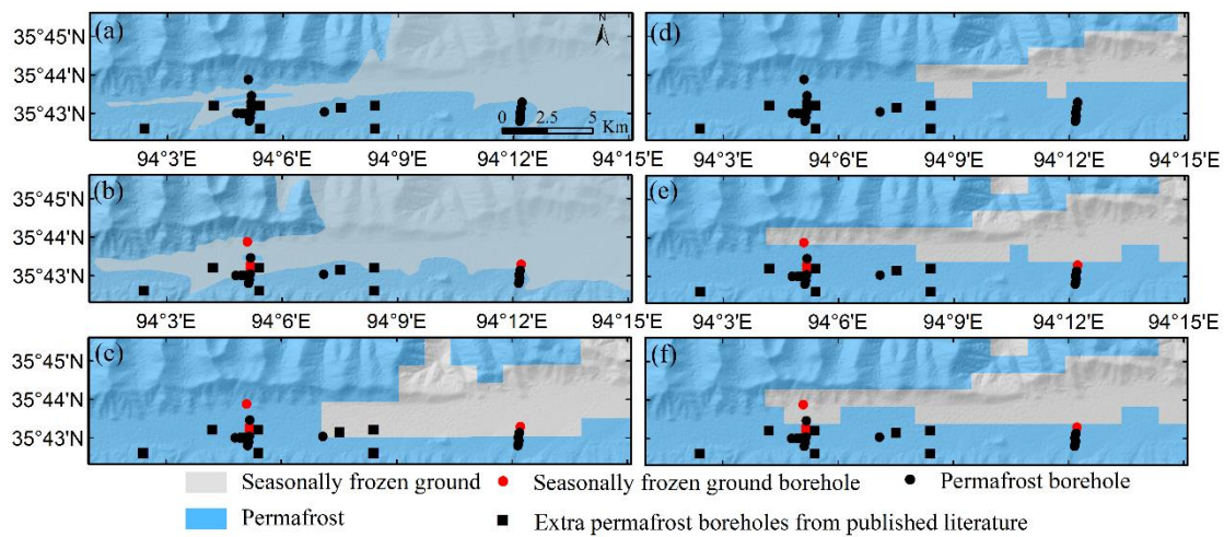
Figure 2. Geographic distribution of permafrost and seasonally frozen ground across the Xidatan for three permafrost maps accomplished in 1975, 2012 and 2016 (left panels 1975 (a), 2012 (b), 2016 (c), published in Nan et al. (2003), Luo et al. (2018) and Zou et al.(2017)) compared to corresponding modelled outputs (right
