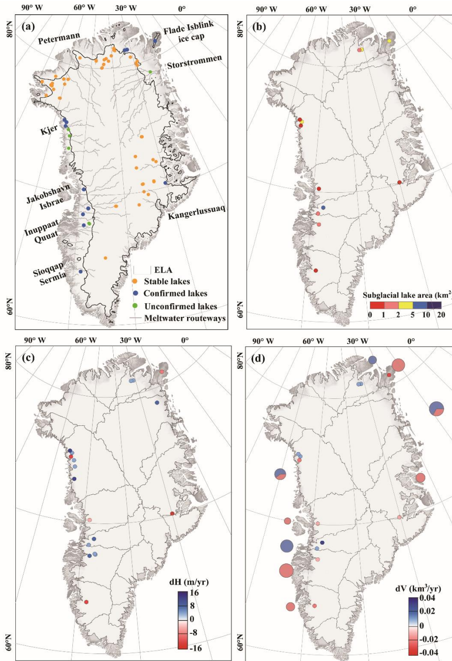
450 Figure 4. Maps of the (a) location, (b) area, (c) elevation change rate and (d) volume change rate during ICESat-2 period for the current active subglacial lakes under the Greenland Ice Sheet. The total lake volume-change rate for each basin is shown as a circle, with the circle size is proportional to the magnitude of the absolute rate in panel (d). Meltwater pathways were derived from the hydraulic gradient (Livingstone et al., 2013). The Equilibrium Line Altitude (ELA) was derived from daily MARv3.12.1 data (Fettweis, et al., 2021). Stable lakes in (a) are from Livingstone et al. (2022).
