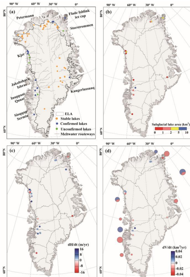
Figure 4. Maps of the (a) location, (b) area, (c) elevation change rate and (d) volume change rate during ICESat-2 period for the current active subglacial lakes under the Greenland Ice Sheet. The pie chart in panel (d) represents the overall volume-change rate of lakes in each basin (blue for positive, red for negative), with the pie size is proportional to the magnitude of the absolute rate. Meltwater pathways were derived from the hydraulic gradient (Livingstone et al., 2013). The Equilibrium Line Altitude (ELA) was derived from daily MARv3.12.1 data (Fettweis, et al., 2021). Stable lakes in (a) are from Livingstone et al. (2022).
