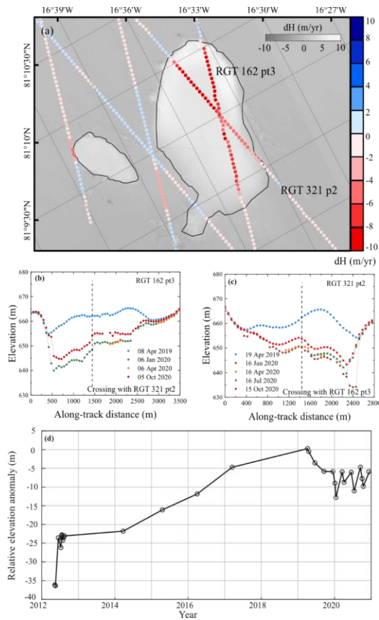
455 Figure 1. Active subglacial lake detection method, using Subglacial Lake ICE_CAPS_NE01 as an example. (a) The elevation 460 change rate was derived from ICESat-2 and overlaid on the elevation difference maps between the two ArcticDEMs (20160923-20160621). The black polygons show the inferred lake boundaries derived from the ArcticDEM. The red-blue spots represent the elevation change rate derived from the linear fit of ICESat-2, while the grayscale colorbar represents the elevation change rate derived from the ArcticDEM. Elevation anomaly profiles across the subglacial lake are given for RGT 162 pair track (pt)3 (b) and RGT 321 pt2 (c). The colors of the points correspond to the ICESat-2 observation times, and the vertical dashed lines show the location of the cross point. (d) Time-series of relative elevation anomaly based on the combined ArcticDEM and ICESat-2 tracks. Note the ~30 m of ice uplift over 6 years that is interpreted to be subglacial lake filling, followed by 10 m of subsidence over 1 year interpreted as slow subglacial lake drainage.
