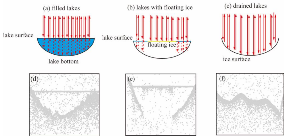
600 Figure 2. Example of how ICESat-2 can penetrate through the water column of supraglacial lakes to measure the lake bottom. The solid and dashed lines indicate strong and weak reflections, respectively. Figure (b) shows an example of a surface lake with floating ice. ICESat-2 can only penetrate the lake surface, but reflects directly off the floating ice. Figure (c) shows an example of a drained lake that ICESat-2 directly measures the ice surface. The second row (d-f) shows examples of the ICESat-2 photon reflection for the corresponding schematic.
