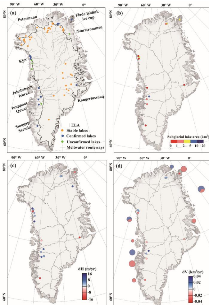
620 Figure 4. Maps of the (a) location, (b) area, (c) elevation change rate and (d) volume change rate during ICESat-2 period for the current active subglacial lakes under the Greenland Ice Sheet. The total lake volume-change rate for each basin is shown as a circle, with the circle size is proportional to the magnitude of the absolute rate in panel (d). Meltwater pathways were derived from the hydraulic gradient (Livingstone et al., 2013). The Equilibrium Line Altitude (ELA) was derived from daily MARv3.12.1 data (Fettweis, et al., 2021). Stable lakes in (a) are from Livingstone et al. (2022).
