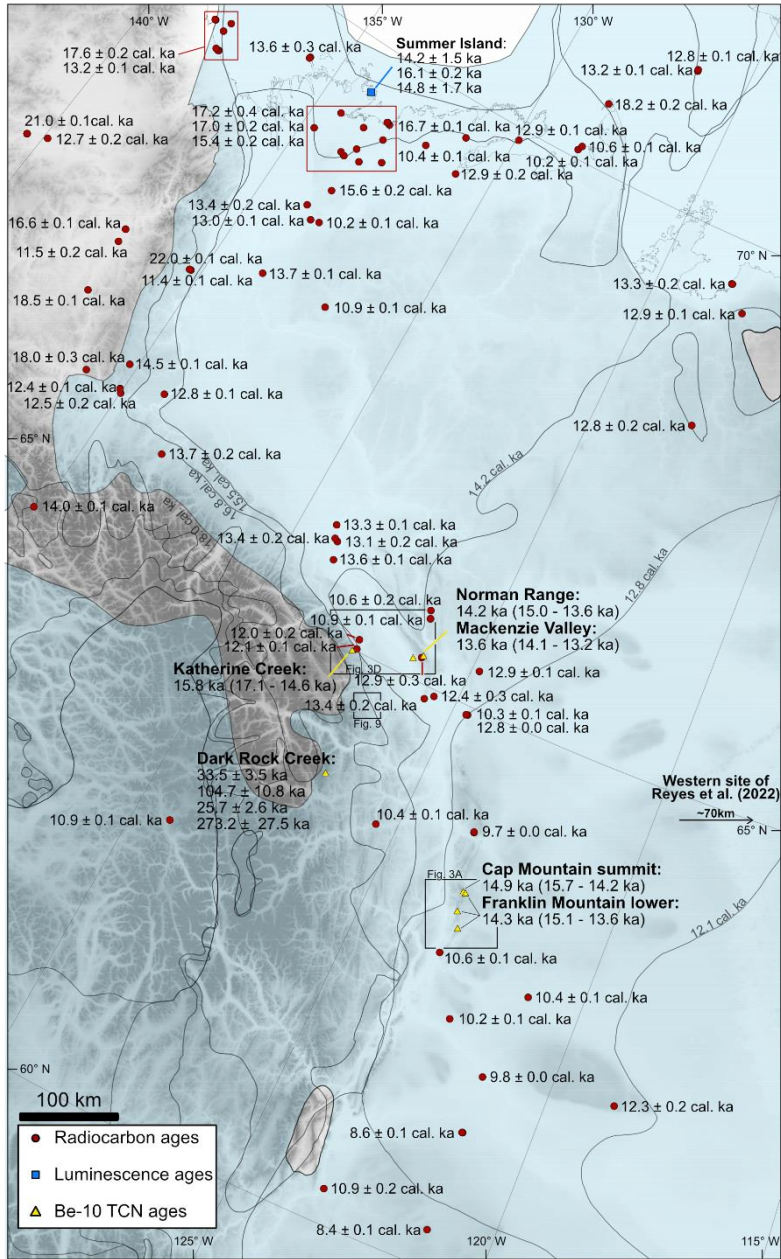
820 Figure 2: The distribution of chronological constraints on the deglaciation of the NW sector of the Laurentide Ice Sheet. The pattern of deglaciation is depicted by grey lines and the shaded blue area represents the local LGM limit at 18.0 cal. ka BP (Dalton et al. , 2020). For our new TCN exposure ages, we present the mean site deglaciation ages ( 2\sigma range) calculated from our Bayesian modelling. Radiocarbon ages were selected from the database of Dalton et al. (2020) and recalculated using the IntCal20 curve (Reimer et al. , 2020). Radiocarbon ages in the red boxes have been grouped together, the ages next to the red boxes are the three
