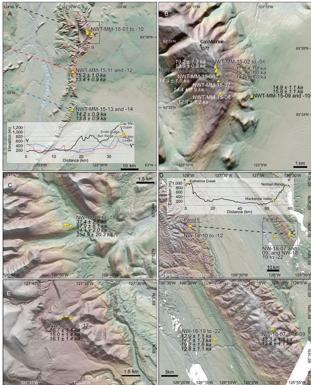
830 Figure 3: (A) Location of the sampling sites in the Franklin Mountains. (B) Close-up of Cap Mountain, where samples NWT-MM-01 to -10 were collected along an elevation transect. (C) Close-up of the Dark Rock Creek site. (D) Location of the northern sampling sites. (E) Close-up of the Katherine Creek site where samples NWT-18-10 to -12 were collected along the ridge. (F) Close-up of the
