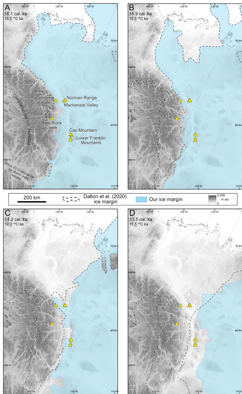
835 Figure 4: . Our ice margin retreat chronology compared to the reconstruction of Dalton et al. (2020). Yellow triangles indicate TCN exposure sampling sites. We do not depict the Cordilleran Ice Sheet in any of our reconstructions (A) Ice margin reconstruction at
