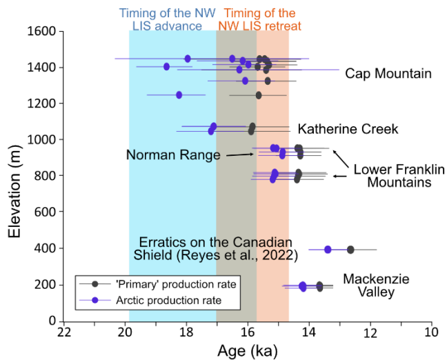
905 Figure 8: The influence of the exposure age calculation approach on the reconstructed age of deglaciation. Shaded orange and blue areas are based on the age constraints in Figure 7. The ‘primary’ production rate exposure ages were calculated using the ‘primary’ calibration dataset (Borchers et al., 2016), LSDn scaling, and a correction for glacioisostatic adjustment (as described in Section 2.1.3) and plotted using the modelled age distribution output of Bayesian model 2 and 5 (Fig. S3 and S4; Table S3 and S4). The Arctic production rate exposure ages were calculated using the Arctic production rate (Young et al., 2013), Lal/Stone scaling, and a correction for GIA (as described in Section 2.1.3) and plotted using the modelled age distribution output of Bayesian model 8 and 11 (Fig. S5 and S6; Table S5 and S6). The wide spread of modelled ages for the Cap Mountain site is a result of the smaller uncertainties associated with exposure ages calculated with the Arctic production rate. 910
