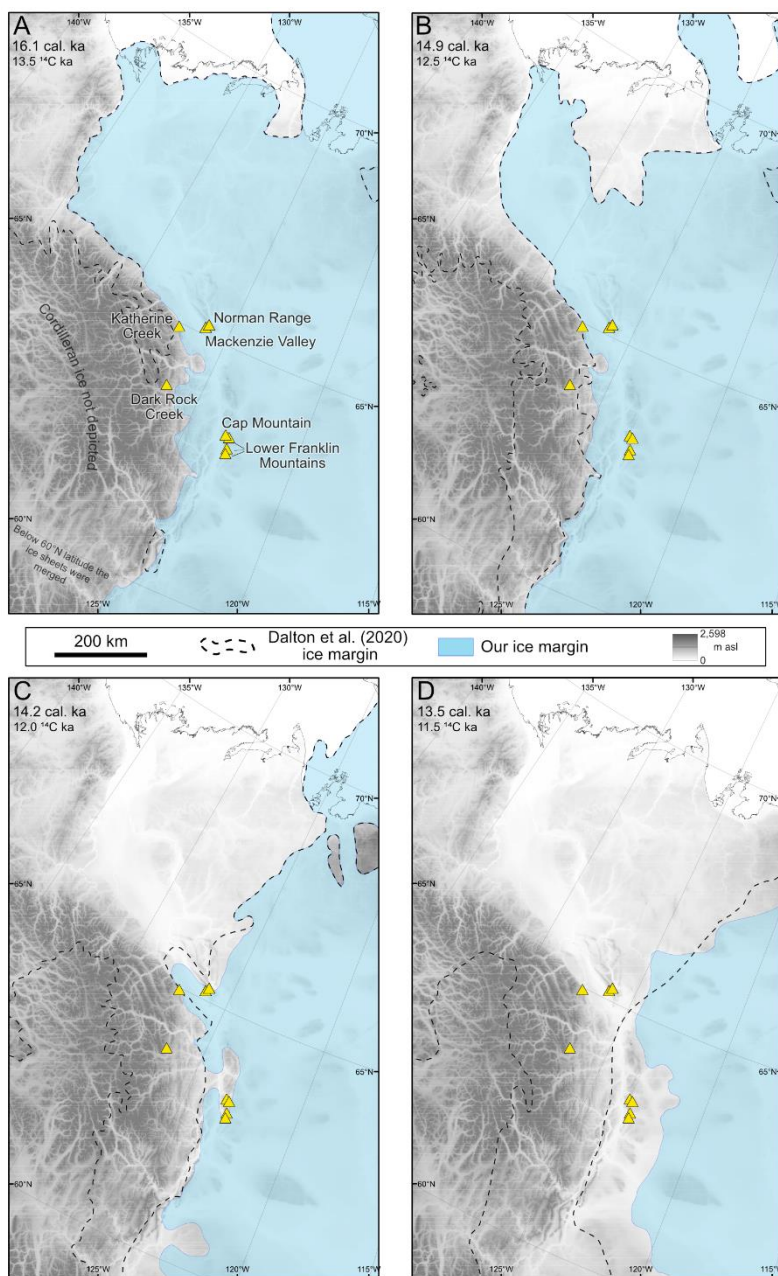
820 Figure 4: . Our ice margin retreat chronology compared to the reconstruction of Dalton et al. (2020). Yellow triangles indicate TCN exposure sampling sites. We do not depict the Cordilleran Ice Sheet in any of our reconstructions (A) Ice margin reconstruction at 16.1 cal. ka. (B) Ice margin reconstruction at 14.9 cal. ka. (C) Ice margin reconstruction at 14.2 cal. ka. (D) Ice margin reconstruction at 13.5 cal. ka.
