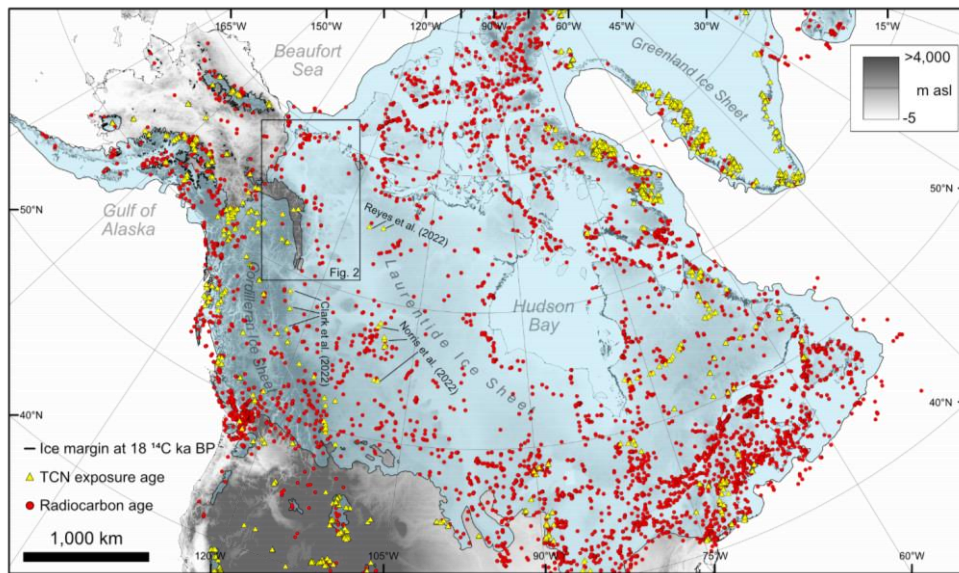
840 Figure 1: The Last Glacial Maximum (18.0 14 C ka/21.1 cal. ka) extent of the North American Ice Sheet Complex according to the reconstruction of Dalton et al. (2020). The yellow triangles ( terrestrial cosmogenic nuclide exposure ages) and red dots (radiocarbon ages) show the distribution of dates constraining deglaciation. The ExPage compilation by Heyman (2022) was used to plot the distribution of terrestrial cosmogenic nuclide exposure ages and the database of Dalton et al. (2020) was used to plot the distribution of radiocarbon ages.
