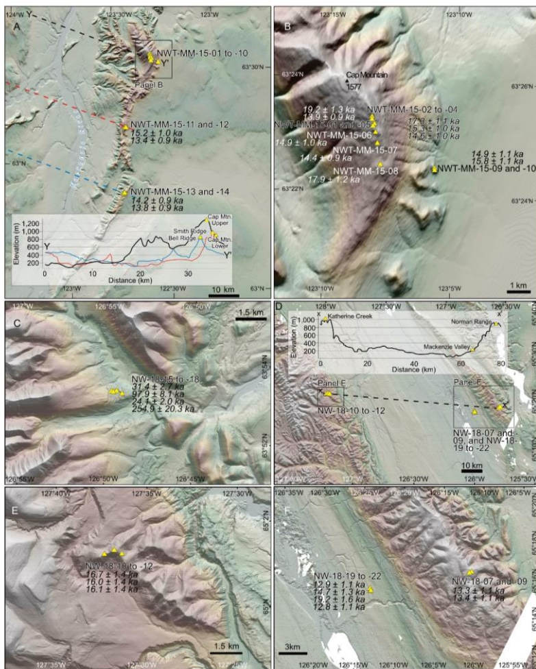
855 Figure 3: (A) Location of the sampling sites in the Franklin Mountains. (B) Close-up of Cap Mountain, where samples NWT-MM-01 to -10 were collected along an elevation transect. (C) Close-up of the Dark Rock Creek site. (D) Location of the northern sampling sites. (E) Close-up of the Katherine Creek site where samples NWT-18-10 to -12 were collected along the ridge. (F) Close-up of the Mackenzie Valley and Norman Range sites where samples NWT-18-19 to -22 and samples NWT-18-07 to -09 were collected. DEM courtesy of the Polar Geospatial Center ( Porter et al., 2018 ).
