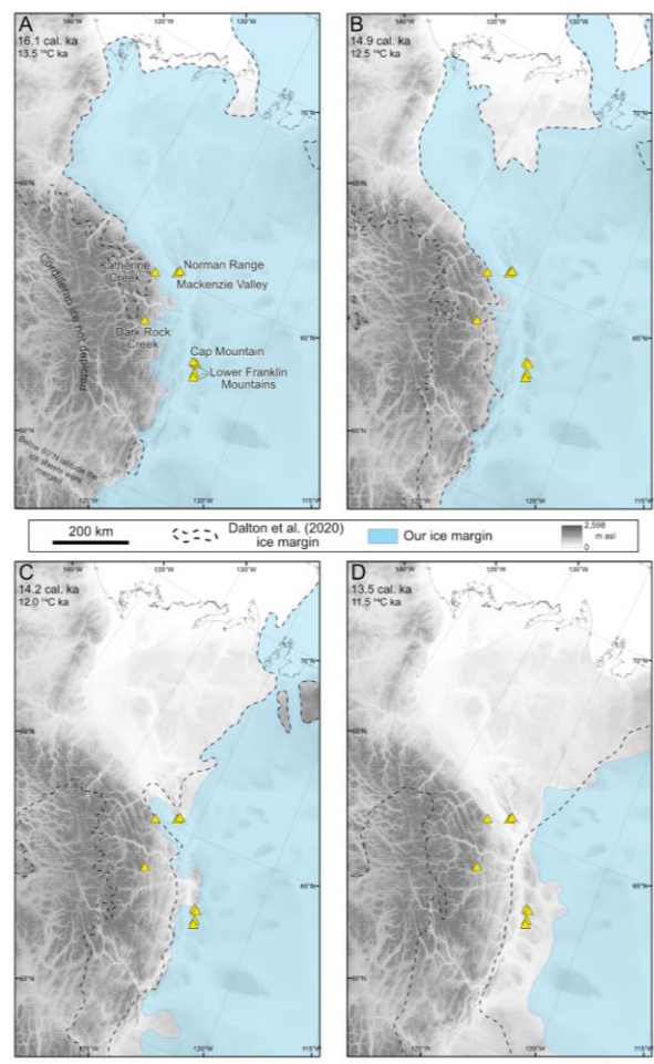
Figure 4: . Our ice margin retreat chronology compared to the reconstruction of Dalton et al. (2020) . Yellow triangles indicate TCN exposure sampling sites . We do not depict the Cordilleran Ice Sheet in any of our reconstructions (A) Ice margin reconstruction at 16.1 cal. ka. (B) Ice margin reconstruction at 14.9 cal. ka. (C) Ice margin reconstruction at 14.2 cal. ka. (D) Ice margin reconstruction at 13.5 cal. ka.
