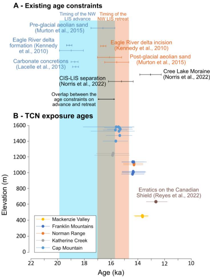
Figure 7: Comparison of our reconstruction of the timing of deglaciation based on the Bayesian model outputs with existing age constraints. The shaded orange area indicates timing of retreat of the NW LIS including dating method uncertainties and the shaded blue area indicates the timing of advance of the NW LIS including dating method uncertainties based on the age constraints in Panel A. (A) Existing age constraints on the timing of NW LIS advance and retreat to the LGM. The chronological constraints of the advance of the NW LIS to the LGM are shown as blue lines and the constraints on the timing of retreat from the LGM are shown in orange. The timing of deglacial events from the multi-chronometer Bayesian model reconstruction of the SW LIS is shown
