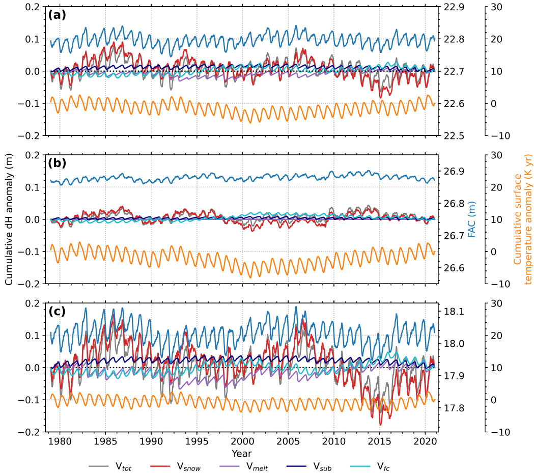
Figure 7. Time series from FDM v1.2A of FAC, of the cumulative anomalies (against long-term mean) of surface temperature, of the vertical firm surface velocity, and of its separate components from Eq. (6). Time series are shown for (a) the entire ice sheet, (b) the part of the ice sheet situated above 2,000 m a.s.l. and (c) the part of the ice sheet situated below 2,000 m a.s.l.
