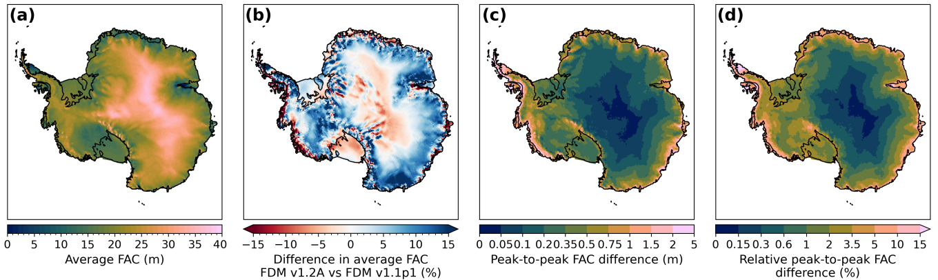
Figure 5. Maps from FDM v1.2A of average (a) firn air content (FAC), (b) the difference in FAC (FDM v1.2A - FDM v1.1p1), (c) peak-to-peak FAC difference, (d) relative peak-to-peak FAC difference compared to the average FAC from (a). The peak-to-peak is defined as the difference between the highest and the lowest FAC value occurring during the study period (1979-2020).
