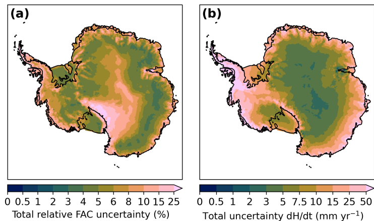
Figure 10. Maps from FDM v1.2A of the estimated ice-sheet-wide total uncertainty in (a) firn air content (FAC) and (b) surface elevation change (dH/dt) from the sensitivity analysis. The FAC uncertainty for all experiments and surface elevation change uncertainty for the spin-up experiments are calculated over 1979-2020, and the surface elevation change uncertainty for the MO fits, \rho_s , T_s and \dot{b} experiments are calculated over 2015-2020.
