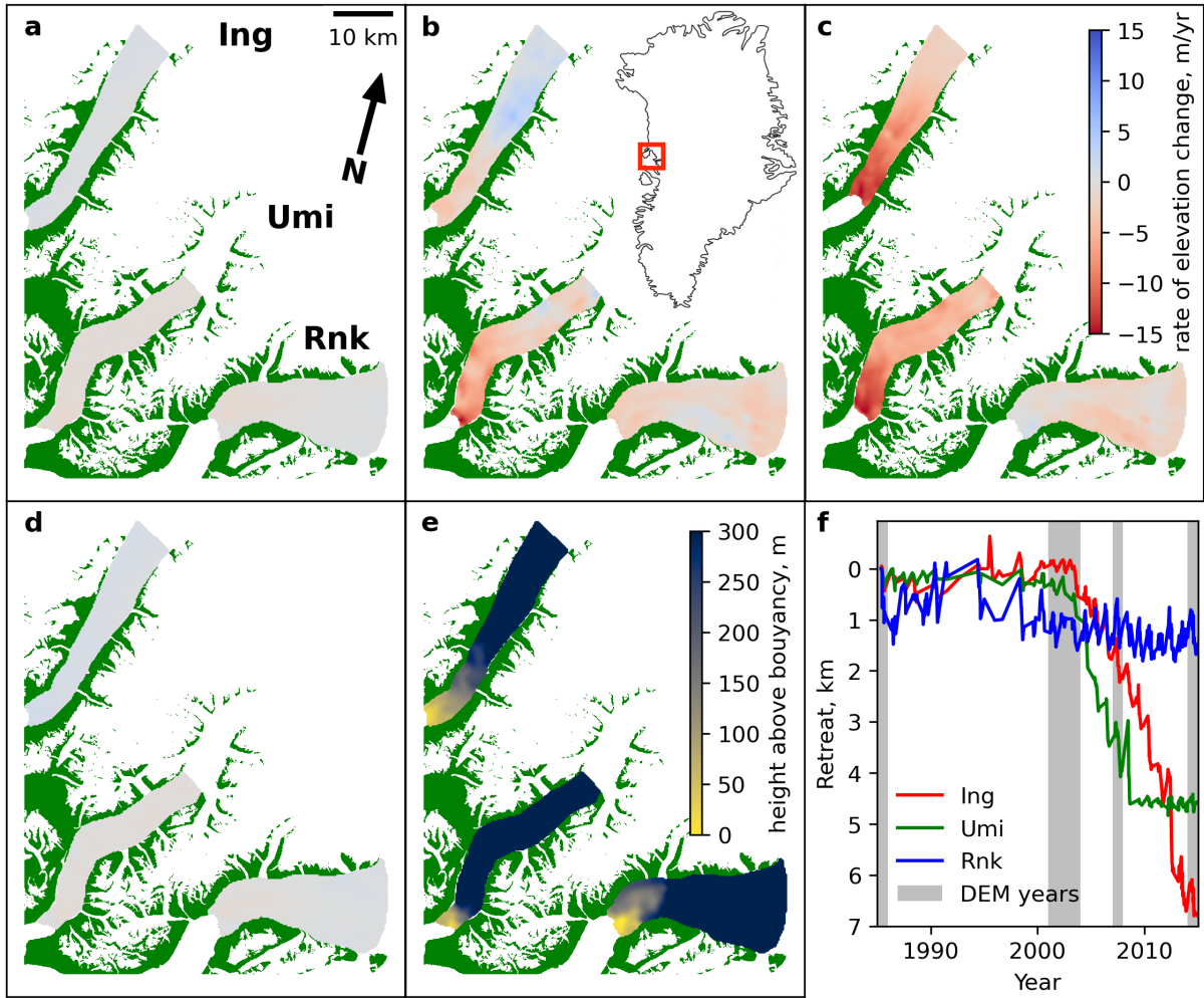
Figure 1. Rate of total elevation change for Ingia Isbrae (Ing), Umiamak Sermia (Umi), and Rink Isbrae (Rnk) from (a) 1985 to ~2002 (Ingia: 2003, Umiamak: 2002, Rink: 2001) (b) ~2002 to ~2007 and (c) ~2007 to ~2015. (d) Dynamic thinning, (total thinning minus thinning from surface mass balance prior to glacier retreat) from 1985 to ~2002. (e) Glacier height-above-buoyancy assuming an open connection to sea level, an ice overburden pressure upper bound, in 1985. In green is the land around the glaciers. All glaciers shown flow from the interior of Greenland on the right hand side of the figures to the ocean on the left where they terminate. (f) Glacier retreat histories since 1985 (Catania et al., 2018), along with dates of DEMs used.
