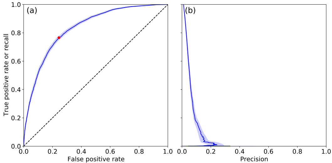
Figure 4. (a) ROC curve for of the test dataset. model trained with all input variables at our spatial resolution and evaluated independently on each winter season since 1958. The optimal point (threshold value of 0.01) is represented by a red dot. (b) Precision and recall (Table 3) curve. Shading represents the uncertainty based on the 20th and 80th percentile of the bootstrap on test evaluation years (see methods section).
