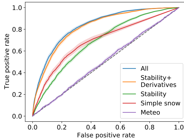
Figure 6. ROC curves of the model trained with different sets of variables. Shading represents the uncertainty by bootstrap on test evaluation years (see methods section). Labels of subsets of variables correspond to those of Table 1. Scores associated to the optimal points (nearest to (0, 1)) are reported in Table 5
