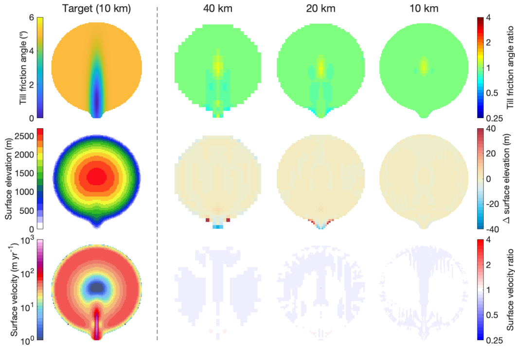
290 Figure 4: Unperturbed inverted bed roughness, surface elevation, and surface velocity in experiment I at different resolutions, compared to the target. Top row: till friction angle; middle row: surface elevation; bottom row: surface velocity. For the target run (first column), absolute values are shown (colour scales on the left); for the three unperturbed inversions (second – fourth columns), errors with respect to the target are shown (colour scales on the right). For the till friction angle and the surface velocity, the ratios between the inverted and the target values are shown, using a logarithmic colour scale.
