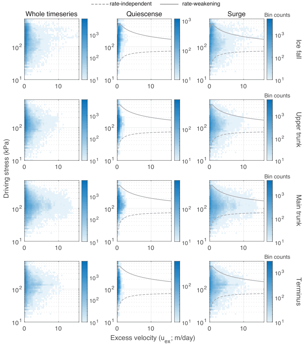
Figure 8. Relationship between driving stress and excess velocities, used as a proxy for sliding velocities. The data on each axis is separated in 40 bins and the plot color represents the number of data points within a bin. Rate-independent and rate-weakening behaviors are shown by the dashed and full lines, respectively. Note that the Y-axis is logarithmic and the X-axis is linear and the effect of axes scaling on data visualization is shown in Figs. S4.8 and S4.9.
