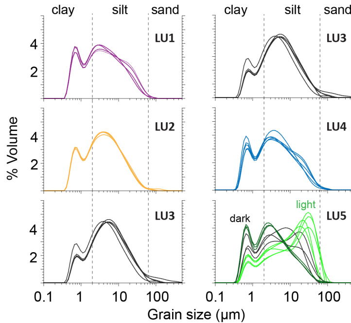
Figure 8. Grain size spectra of lithologic units 1 – 5 illustrating the similar grain size distributions of sediments in LU1 and LU4, as well as the difference between the dark (less dense) and light (more dense) laminations in LU5.
