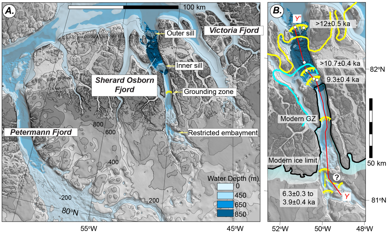
575 Figure 12. A. Bathymetry and sub-glacial topography of north Greenland from Morlighem et al. (2017) illustrating pronounced differences between the broad submarine trough that extends inland from Petermann Glacier and the more restricted, and rapidly shoaling topography in Sherard Osborn and Victoria Fjords. B. Detail of Sherard Osborn Fjord showing the two mapped sills that correspond to the likely grounded limits of Ryder Glacier during the Kap Fulford and Warming Land Stade. At the end of the Middle Holocene, Ryder Glacier likely retreated to a more inland position becoming largely land-based and cut off from the main fjord by the restricted embayment. White dots are the coring sites discussed in the text. Red line (Y-Y') shows the position of the bathymetric profile used in Fig. 11. The bathymetry of Sherard Osborn Fjord has been updated from Bedmachine V3 including the incorporation of multi-beam mapping data from Ryder 2019 (Supplementary Figure S10). Ice margin positions during the Kap Fullford Stade (yellow line) and Warming Land Stade (blue line) are from Kelly and Bennike (1992). GZ = Grounding Zone. 580
