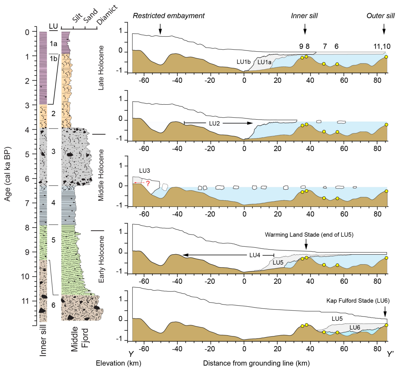
510 Figure 11. Generalised lithology and corresponding reconstructions of Ryder Glacier and ice tongue during deposition of the lithologic units. The profile location is illustrated in Fig. 11. The bathymetry was re-gridded from BedMachine v3 (Morlighem et al., 2017) after adding bathymetric data collected on Ryder 2019 . Substantial modifications to the former digital elevation model exist around the now mapped inner sill and beneath the modern ice tongue (see supplementary material for details). Yellow dots indicate approximate positions of coring stations discussed in the text.
