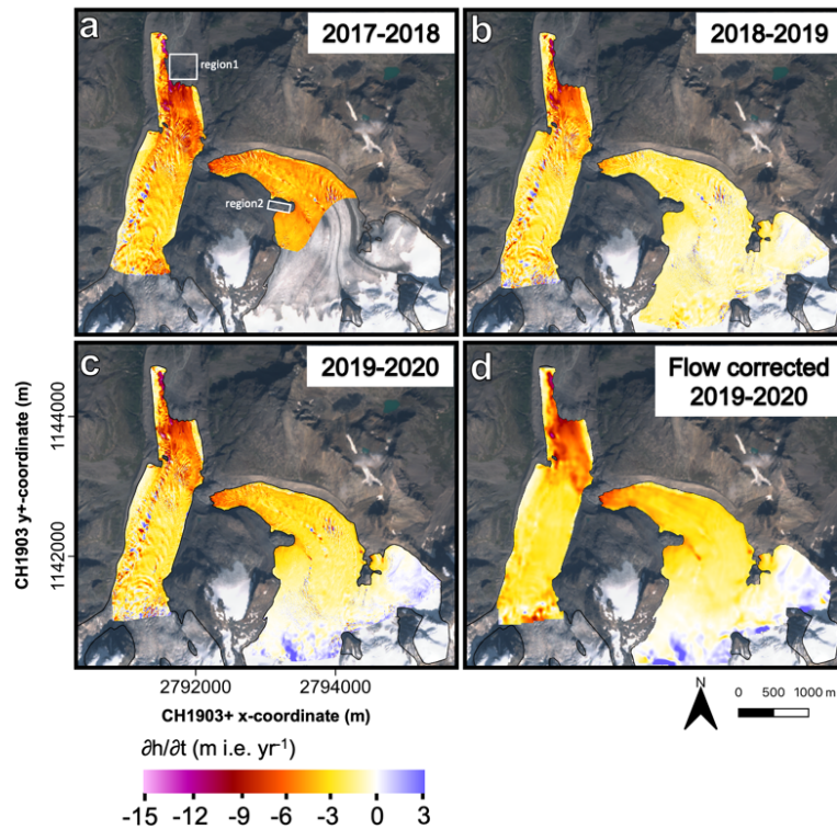
625 Figure 4. Surface elevation changes for (a) 2017-2018, (b) 2018-2019 and (c) 2019-2020. The spatial resolution is equal to 8 626 cm. Panel d shows the surface elevation changes for 2019-2020 after flow correction. The outline of the glacier corresponds 627 to the latest year of observation for every balance year in consideration. The two white boxes (region 1 and region 2) are stable 628 areas which are used for the error analysis. The background image is a Sentinel-2 true colour composite satellite image from 629 13 September 2020.
