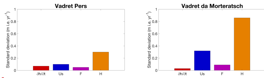
Figure 13. Standard deviation of the MAE for the perturbed versions of the surface elevation changes, the surface velocity ( u_s ), the F-value and the ice thickness (H).
