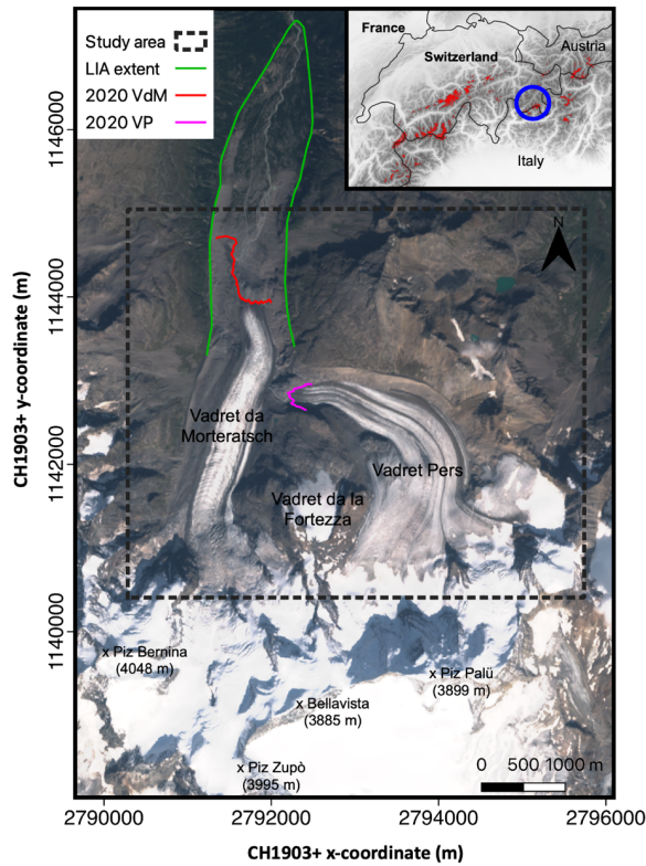
Figure 1 Map of the Morteratsch-Pers glacier complex in southeastern Switzerland. The different coloured lines represent the extent of the glacier at the end of the Little Ice Age (LIA, 1860-1865) and in 2020. The background image is a Sentinel-2 true colour composite satellite image from 13 September 2020. The highest mountains are labelled and indicated with a black cross. The inset shows a DEM of the Shuttle Radar Topography Mission (SRTM) and boundaries of the countries of the central and western European Alps. The areas indicated with a red colour are glaciers according to the Randolph Glacier Inventory (RGI) version 6. The location of the Morteratsch-Pers glacier complex is indicated with a blue circle.
