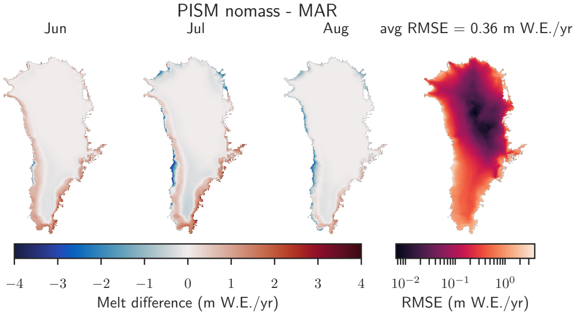
Figure 2. Local differences between the monthly averaged June, July, and August melt rates as diagnosed with PISM-dEBM-simple compared to MAR. The PISM simulation uses monthly 2D temperature fields from MAR as forcing and parametrizes albedo and shortwave downward radiation as detailed in 2.3.1 and 2.3.2. Positive numbers mean that PISM overestimates the melt and negative numbers mean that PISM underestimates the melt. The local root mean square error averaged over June, July and August from 1958-2019 is shown in the right plot. The spatial average of the RMSE is 0.36 m/yr.
