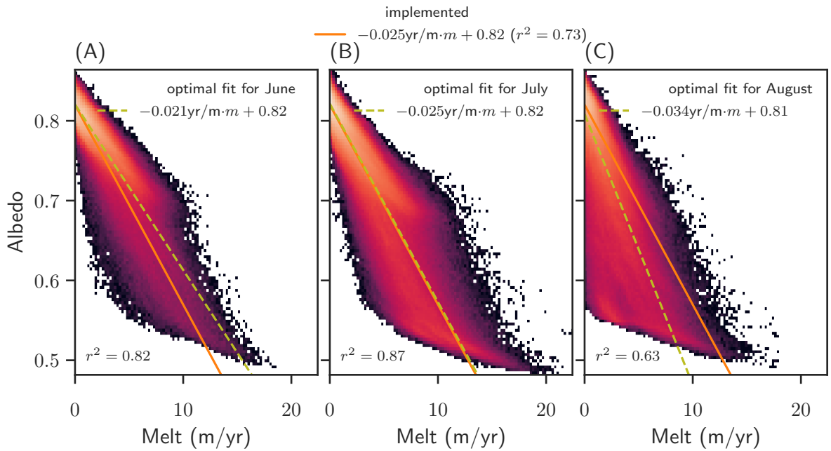
Figure A1. Fit for albedo parametrization Albedo-Histograms of albedo vs. melt of in June (A), July (B), and August (C) over the period 1958 - 2019 in the MAR v3.11 dataset. Each dot represents Colors represent how often the combination of values is found in one each grid cell of on the ice sheet, averaged over a month the years. Note that the color scale is logarithmic. Orange lines show the parametrization with parameters as used in PISM. Light green lines show the best linear fit for each month, with the parameters given in the legend.
