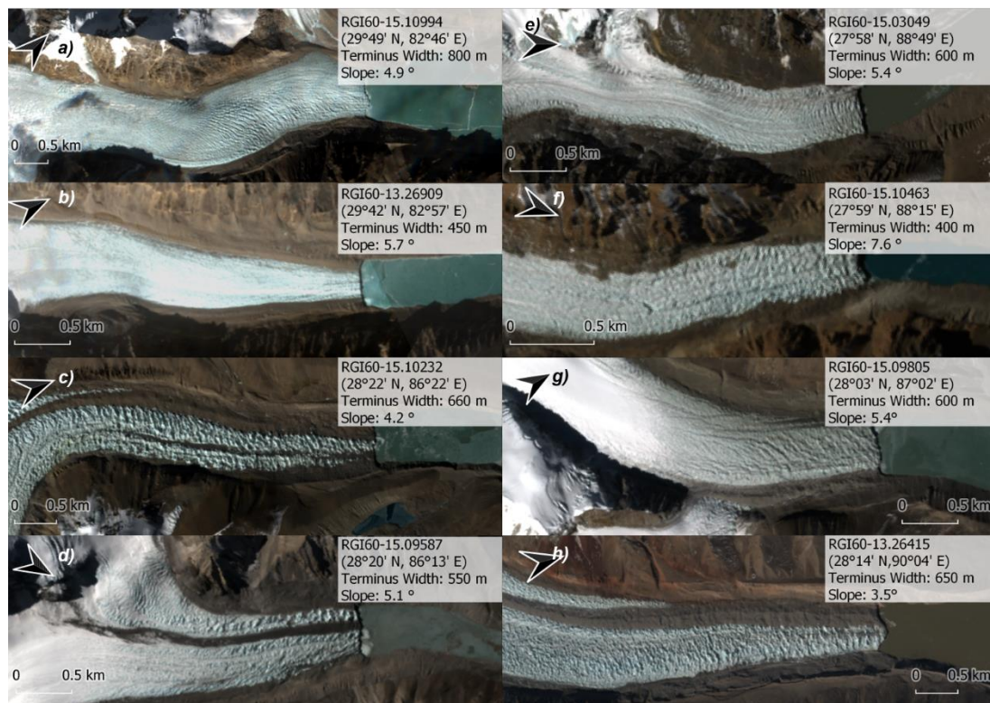
680 Figure A1: Examples of lake-terminating glacier with glacier attributes within 2 km of the terminus. RGB images are retrieved from Sentinel-2.
