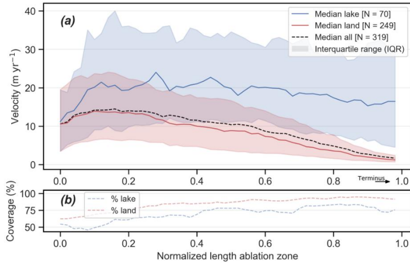
Figure 5: Median centre flow line surface velocity (m yr -1 ) (a) and coverage (%) of the velocity estimates (b). (a) The spread of the velocity along the centre flow line among the glacier population is represented by the IQR. (b) The coverage is defined by the percentage of valid velocity estimates ( CI_{95} < 5 \text{ m yr}^{-1} ) at a given position along the centre flowline.
