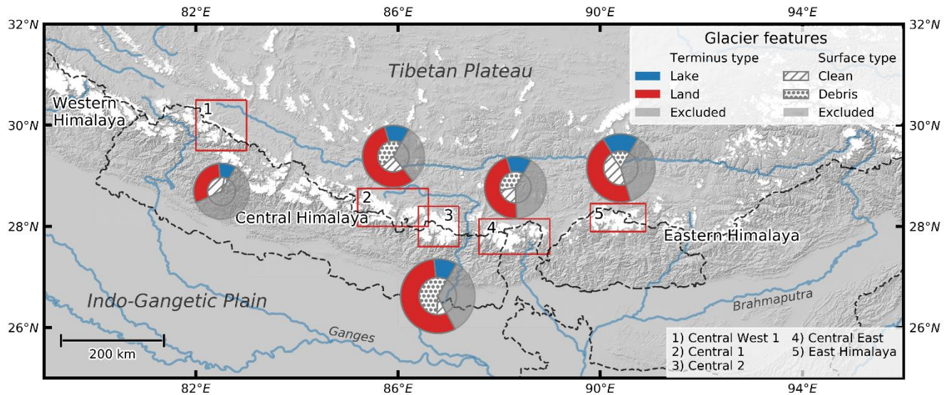
Figure 1: Map showing the regional subdivisions (red rectangles) with the associated glacier characteristics, including terminus type and surface cover as a fraction of the total sub-regional glacierised area. The excluded fraction represents the glacierised area from glaciers smaller than 3 \text{ km}^2 . The names of the subregions are in accordance with King et al. (2019). Country boundaries are tentative and for orientation only. This figure was generated using Matplotlib 3.1.2, together with Python 3.7.
