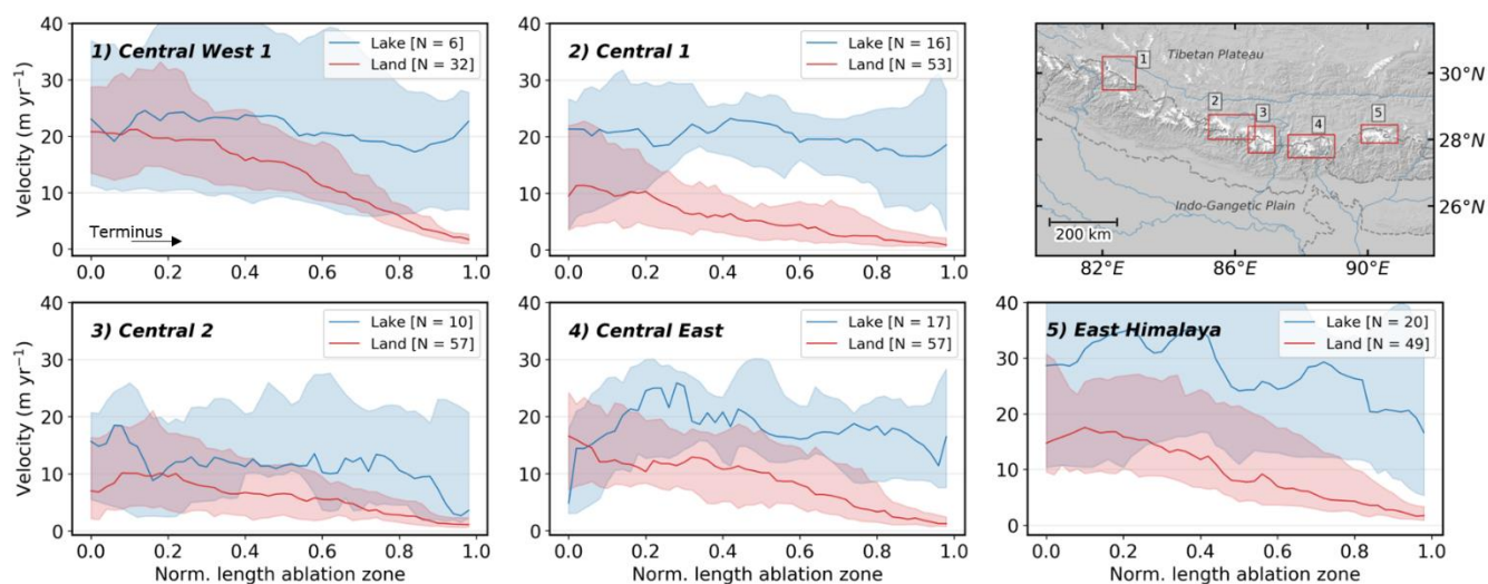
445 Figure 7: Subregional glacier median centre flow line velocity estimates and their location along the CE Himalaya (red rectangles). The spread of the velocity along the centre flow line among the glacier population is represented by the IQR, with the number of glaciers shown in the legend between the brackets. This figure was generated using Matplotlib 3.1.2, together with Python 3.7.
