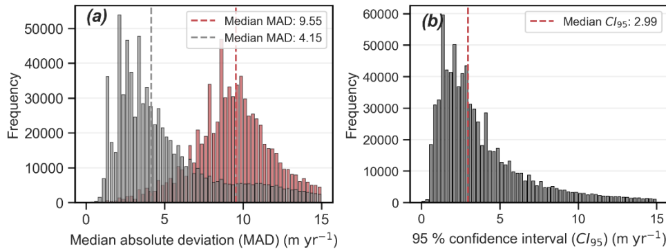
330 Figure 2: Dispersion ( MAD_{disp} ) (a) and 95 % confidence interval ( CI_{95} ) (b) of the velocity estimates at glacierised areas. (a) The red distribution represents the MAD_{disp} before subtracting V_{off} from each image pair, which realised a 56% reduction of the median dispersion, resulting in the grey dispersion distribution. (b) CI_{95} resulting from the estimated distribution of median displacement vector as a function of the number of velocity estimates and MAD_{disp} (Eq. 2).
