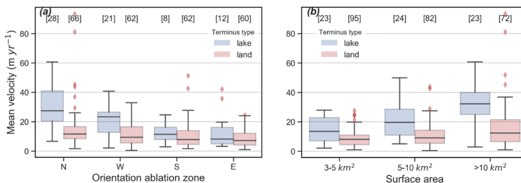
420 Figure 6: Boxplot showing the mean velocity contrast between lake-terminating and land-terminating glaciers depending on the orientation of the ablation zone (a) and surface area (b). The IQR (boxes) represents the spread within the mean sample group. Points outside of the 3rd quartile plus 1.5 times the IQR range are plotted explicitly.
