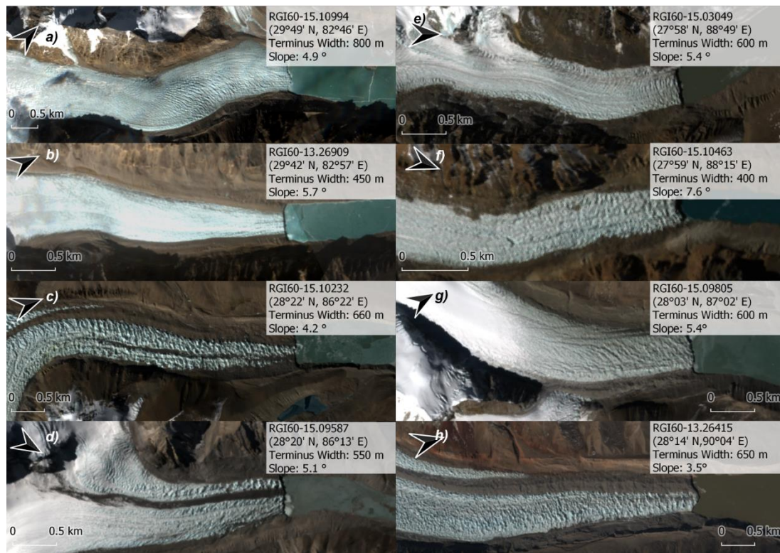
675 Figure A1: Examples of lake-terminating glacier with glacier attributes within 2 km of the terminus. RGB images are retrieved from Sentinel-2.
