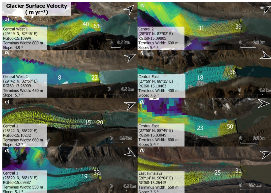
560 Figure 11: Examples of lake-terminating glacier accelerating towards their terminus with glacier attributes within 2 km of the terminus. White numbers represent the glacier surface velocity in m yr -1 . Colour scale of plotted velocity data is indicative and varies among glaciers. Velocity data and RGB images are retrieved from Sentinel-2.
