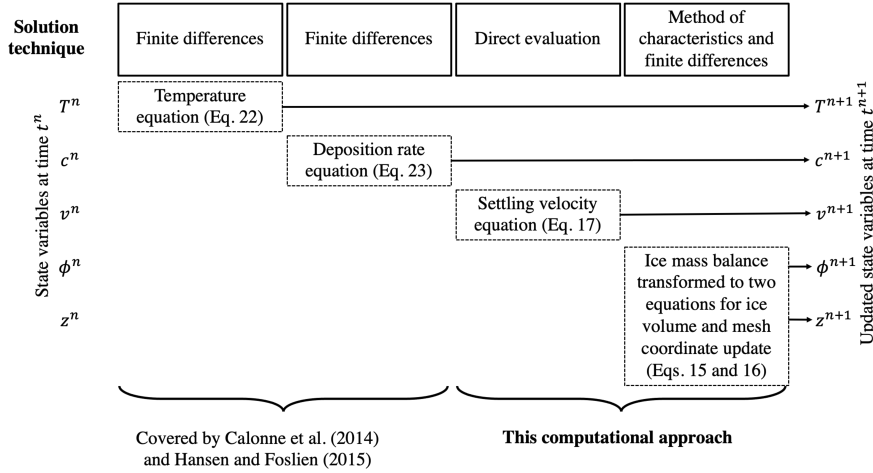
Figure 2. Illustrates the computational workflow of one iteration. The state variables at time t^n , depicted on the left hand side, are updated through the modules annotated as dashed boxes, and that are ordered diagonally in the centre of the figure. After each update the state variables at time t^{n+1} are retrieved. The equations of the modules are implemented into the computational model through the respective solution technique stated in the solid boxes on the top row. The computational steps are carried out from top to bottom. The equations for heat and vapor transport have already been implemented by Calonne et al. (2014) and Hansen and Foslien (2015). iterative approach can be summarized as: 1) determine time step size \Delta t according to Eq. A-feedback (25), 2) update the temperature field based on Eq. (21), 3) compute the ice volume fraction in deposition rate with the absence of a vertical velocity has been investigated in the companion paper (?) temperature field based on Eq. The modules for (22), 4) determine the vertical velocity with Eqs. (17) and for the coupled (18), and 5) update of the ice volume fraction and the mesh coordinates simultaneously based on Eqs. (3.3) and (3.3). While 2) and 3) is a re-implementation of an existing approach previously published by Hansen and Foslien (2015); Calonne et al. (2014), through their coupling to 4) and 5) constitutes the method novelties of characteristics our work. Note that 4) is novel computed as part of 5) in our approach the code.
