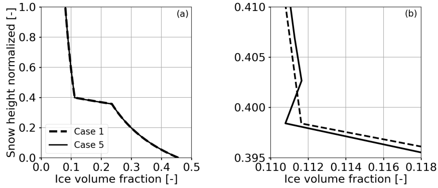
Figure 8. The plots show ice volume fraction profiles over normalized snow height after 2 days. The dashed line (a) depicts ice volume fraction for Case 1 of (Table 2) depicts ice volume fraction corresponding to solely active settling, whereas the solid line depicts ice volume fraction computed based on and Case 5, which refers to the fully coupled processes. (b) zooms into the density transition area of (a) and. The kink in the profile of Case 5 shows the effect of the increased sublimation in Fig. 7 on that yields a local decrease in ice volume fraction. In order to better resolve the kink of Case 5, we increased the number of grid nodes to 251.
