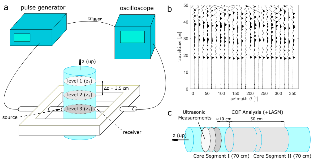
Figure 1. (a) Schematic experimental setup for ultrasonic measurements on the ice core with tools and devices (amplifiers not shown). (b) Example dataset of seismic traces for horizontal measurements. (c) The segmentation of two adjacent ice core segments depicting the position of the ultrasonic and COF analyses.
