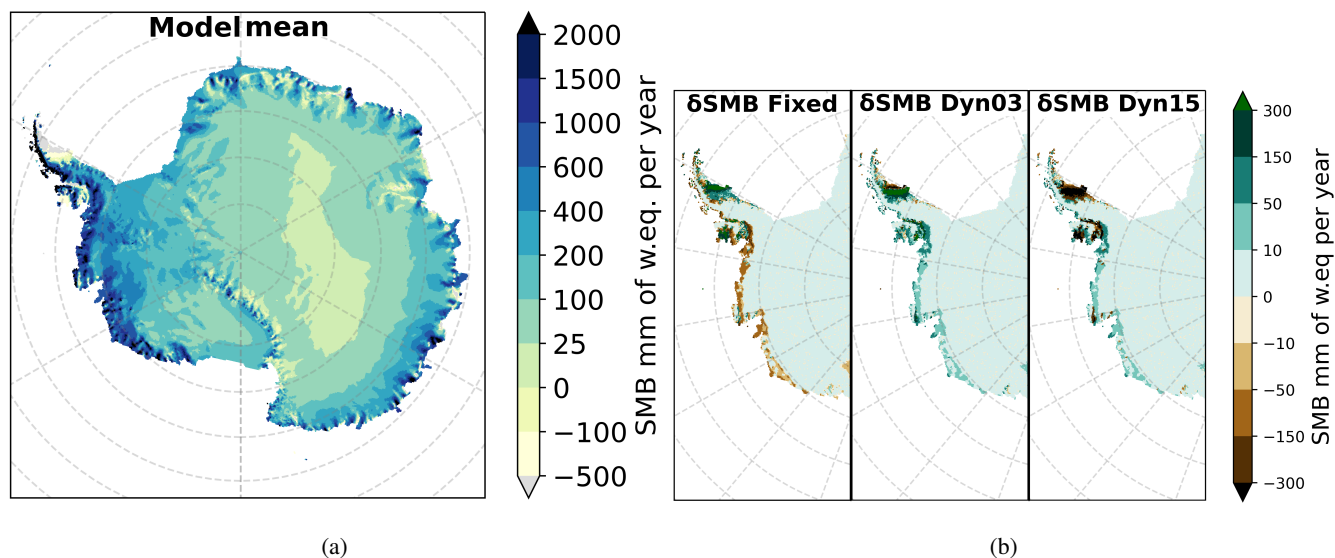
Figure 1. Mean SMB from 1980 to 2017 in mm yr -1 of w.eq.. a) the mean of the model mean, note nonlinear colour bar. b) West AIS where the \delta SMB has the largest differences between model versions, (model minus ensemble mean).
