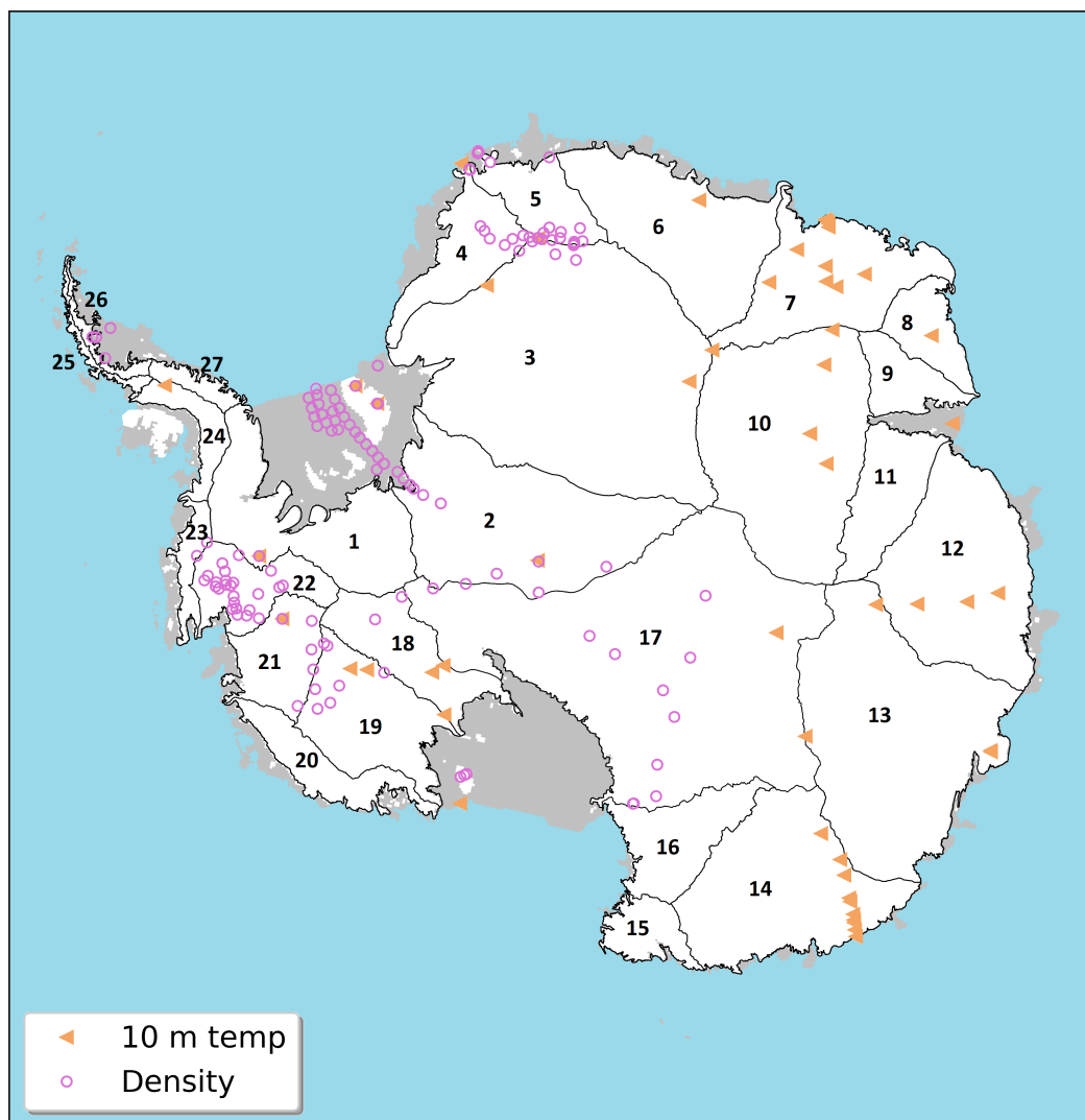
Figure 4. The white colour shows the GAIS and the gray colours show the locations of ice shelves. The spatial distribution of observations are shown with light brown triangles for borehole temperatures and magenta circles for the location of the density profiles. The grounded basins are derived from Zwally et al. (2012) and outlined by black lines.
