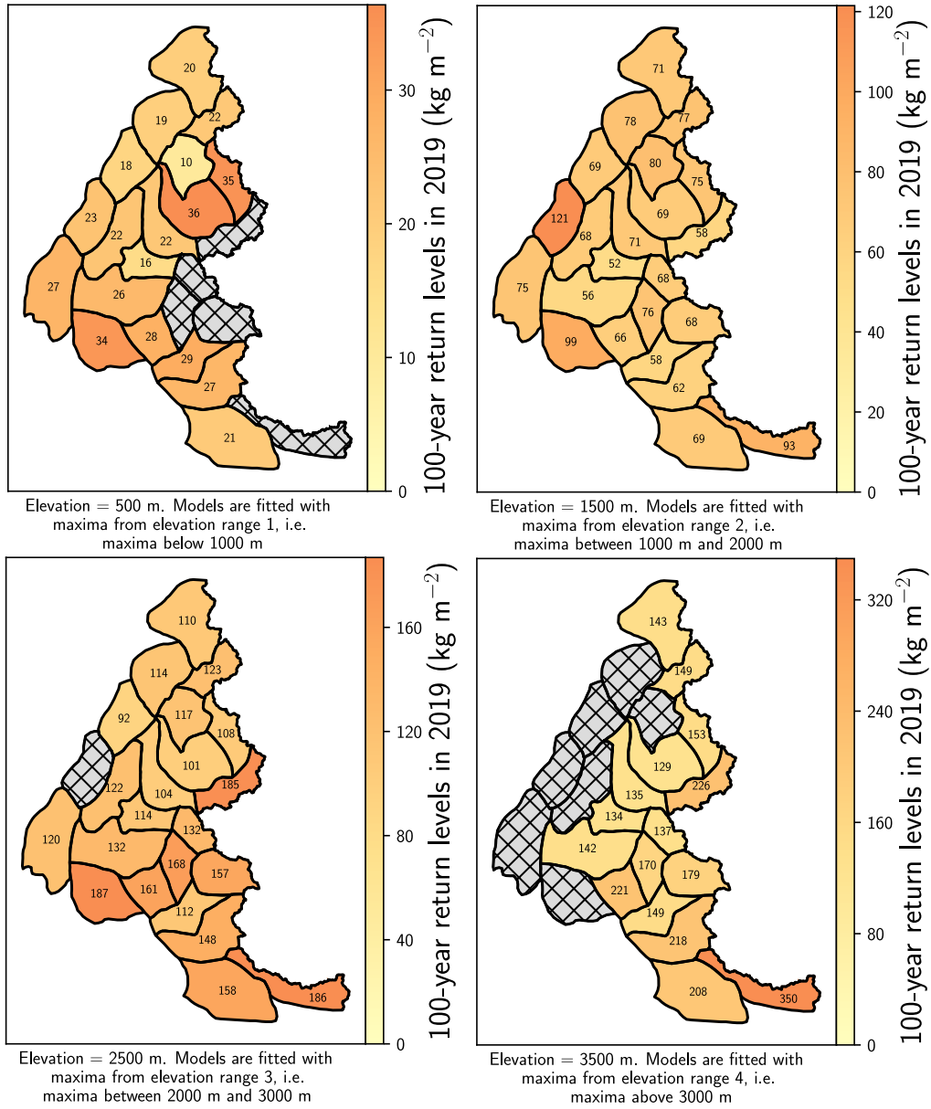
Figure 9. 100-year return levels in 2019 of daily snowfall for each range of elevations. 100-year return levels are both illustrated with colours (elevation range dependent scale) and written on the map. Hatched grey areas denote missing data, e.g. when the elevation is above the top elevation of the massif. Return levels are computed at the middle elevation for each range, e.g. at 1500 m for the range 1000-2000 m
