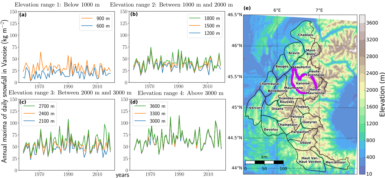
Figure 1. (a, b, c, d) Time series of annual maxima of daily snowfall from 1959 to 2019 for the Vanoise massif (purple region) clustered by the four ranges of elevations considered. (e) Topography and delineation of the 23 massifs of the French Alps (Durand et al., 2009).
