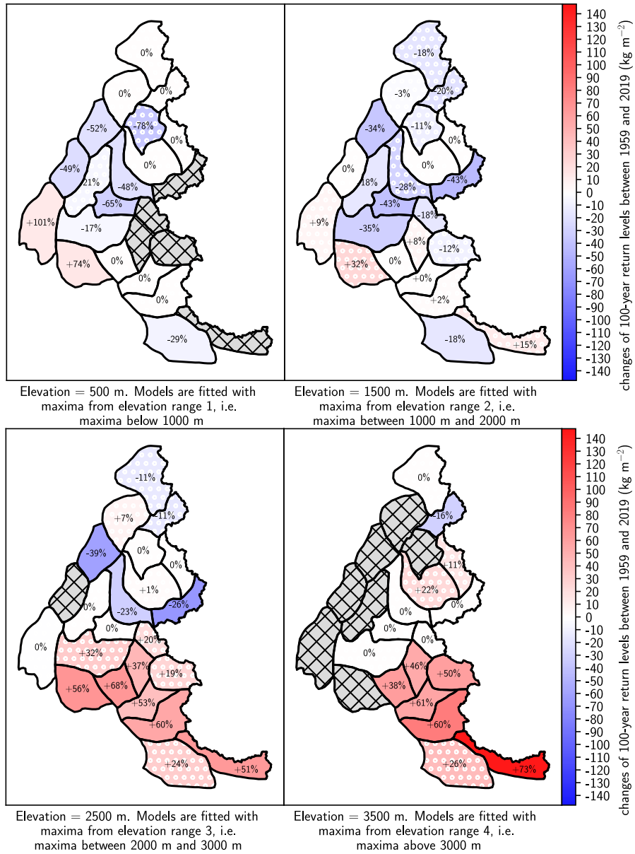
Figure 8. Changes of 100-year return levels of daily snowfall between 1959 and 2019 for each range of elevations. The corresponding relative changes is written are displayed on the map. Hatched grey areas denote missing data, e.g. when the elevation is above the top elevation of the massif. Changes of return levels are computed at the middle elevation for each range, e.g. at 1500 m for the range 1000-2000 m. Massifs with non-significant trends are indicated with a white-dotted pattern.
