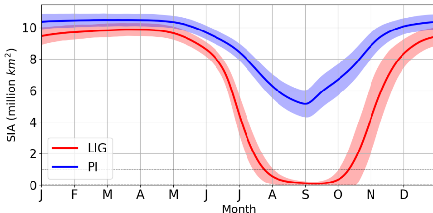
Figure 1. Annual cycle of Arctic sea-ice area (SIA). The 200-year mean calculated from daily model output from 70^\circ\text{N} - 90^\circ\text{N} for the LIG (red) and PI (blue) simulations is shown.
