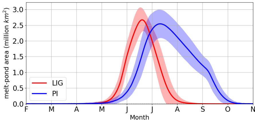
Figure 10. Annual cycle of Arctic melt pond area. The 200-year mean was computed from daily model output variables grid-cell sea-ice area and melt pond area, over the region from 70°N - 90°N. Shaded area is \pm twice the standard deviation. Only ice-covered grid-cells were used.
