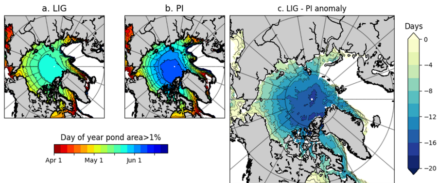
Figure 8. First day of melt pond formation as proxy for melt onset. The mean day of the year the grid-cell melt pond fraction grew above 0.01 for (a) LIG, (b) PI, and (c) the LIG - PI anomaly. All figures show the 200-year mean, from daily model output. Only grid-cells still ice-covered when melt ponds began to form are shown.
