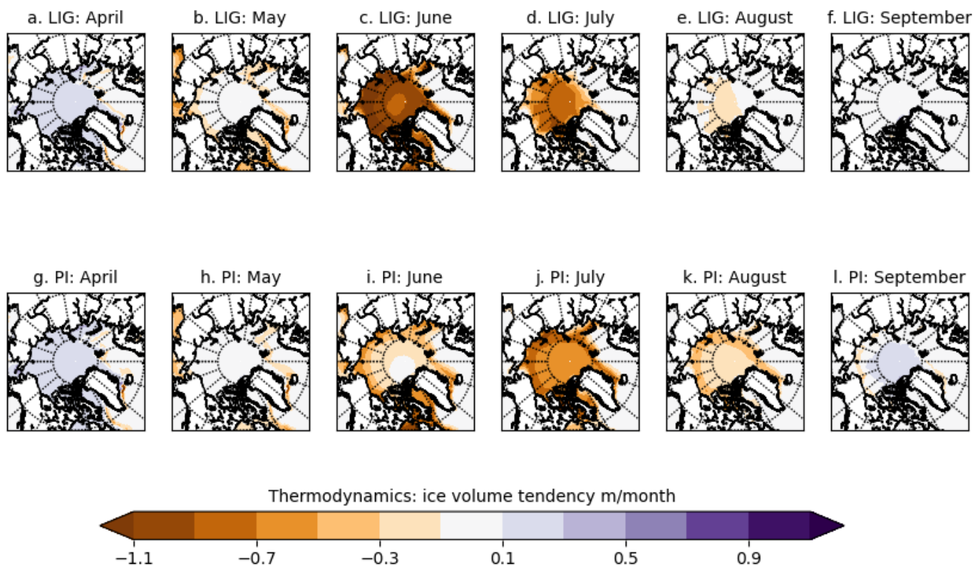
Figure 6. Maps of mean simulated ice volume tendency [m/month] due to thermodynamics, for the LIG and PI. The 200-year mean over the Northern Hemisphere for each month from April-September is shown, computed as the time-average from monthly model output.
