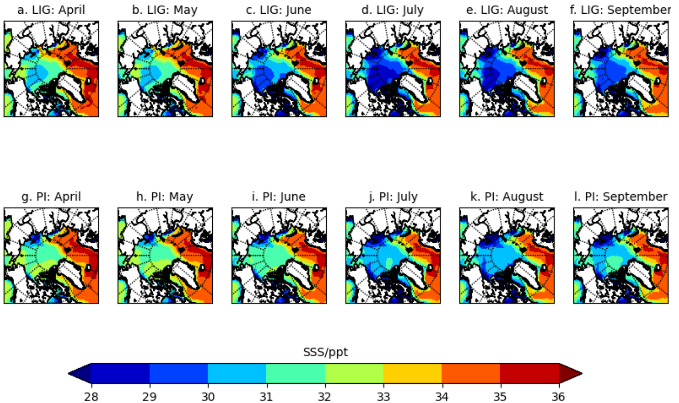
Figure 3. Mean sea surface salinity (in parts per thousand, ppt), for the LIG and PI. The 200-year mean over the Northern Hemisphere for each month from April-September is shown, computed as the time-average from monthly model output.
