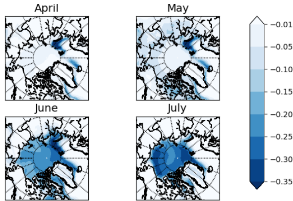
Figure 7. The LIG-PI albedo difference. For both LIG and PI, the albedo for each grid-cell was computed from monthly model output variables absorbed and downwelling short-wave flux. The LIG-PI anomaly is computed from the 200-year time averages for the PI and LIG.
