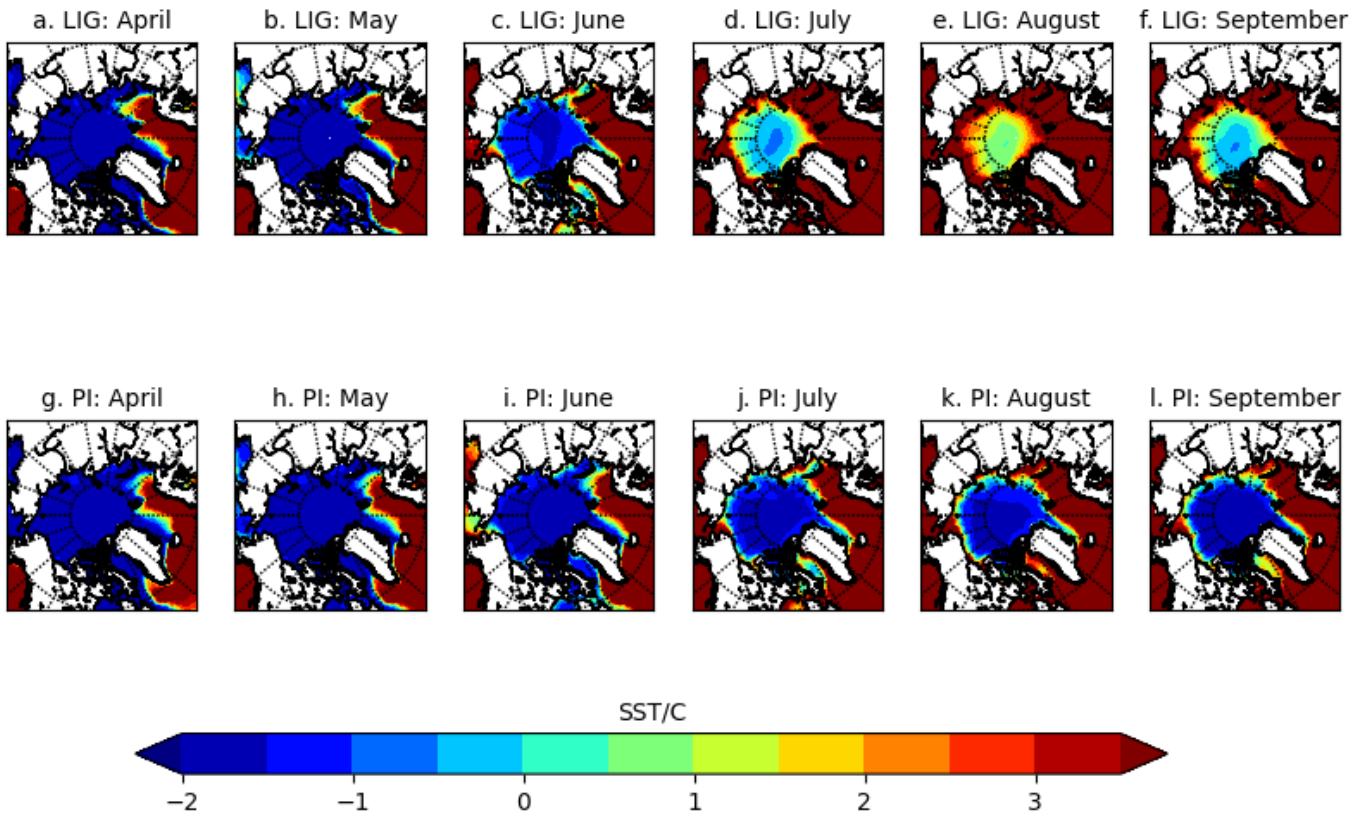
Figure 2. Mean sea surface temperature °C, for the LIG and PI. The 200-year mean over the Northern Hemisphere for each month from April-September is shown, computed as the time-average from monthly model output.
