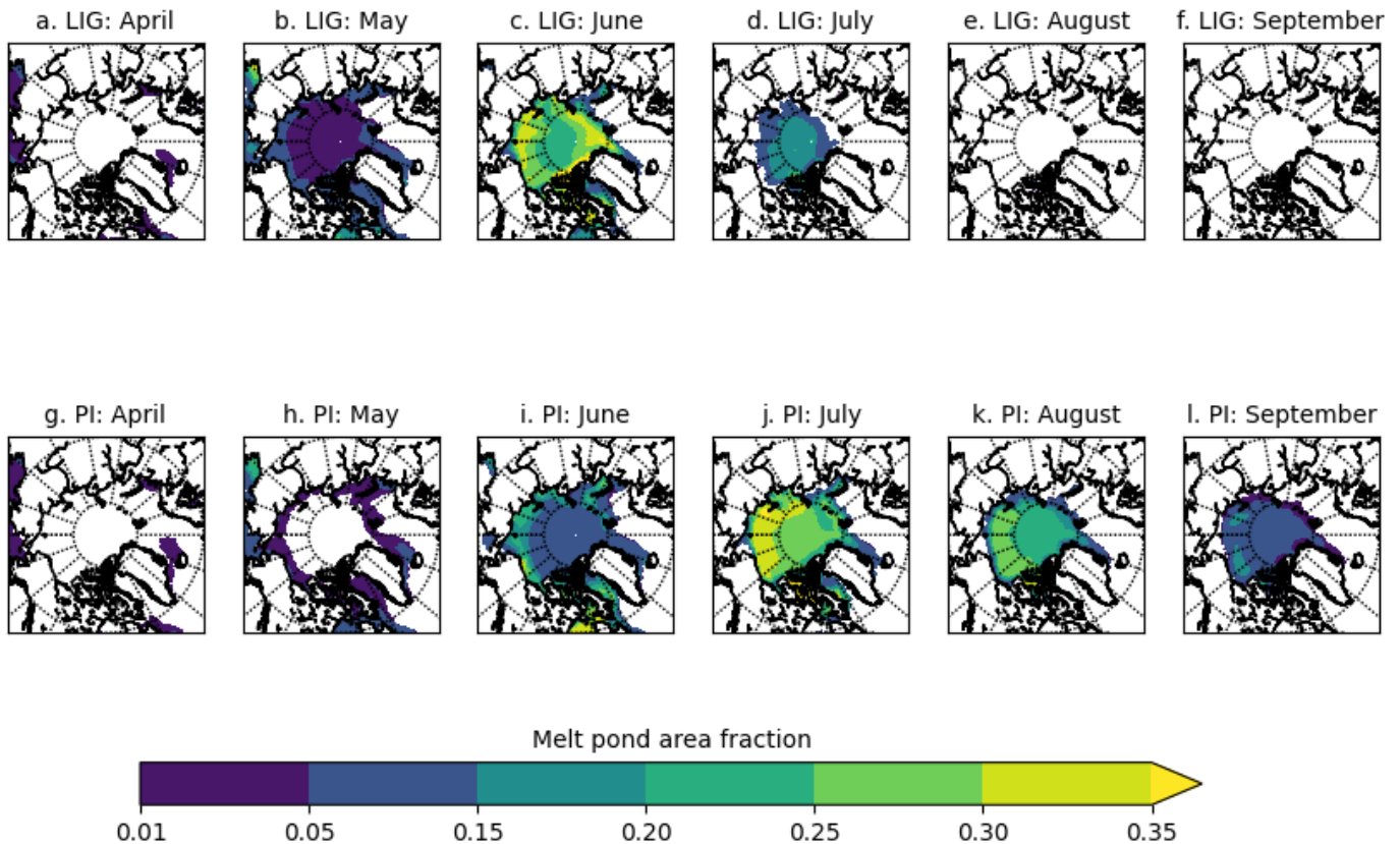
Figure 9. Melt pond fraction. Monthly simulated melt pond fraction of the grid-cell for LIG and PI. The 200-year mean over the Northern Hemisphere for each month from April-September shown is the time-average from monthly model output.
