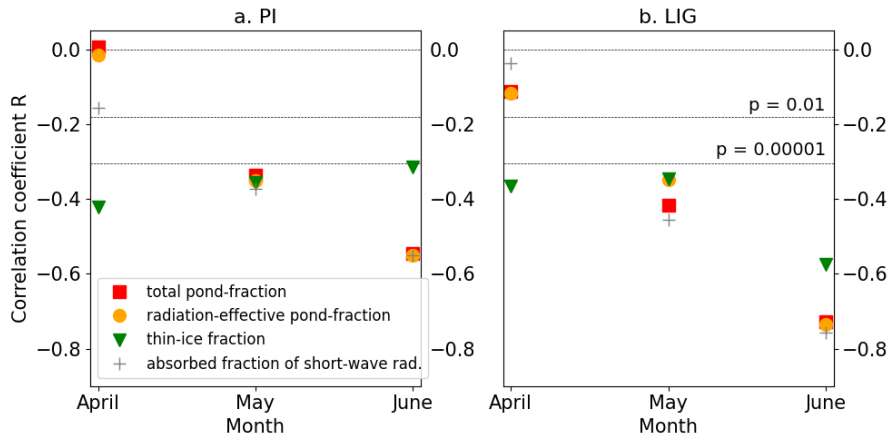
Figure 12. Correlation between spring melt pond fraction (MPF) of sea-ice area (SIA) and autumn SIA for (a) PI, and (b) LIG. For both (a) and (b), 200 years of monthly model data were used over the region 70°N - 90°N. Pearson's correlation coefficient R was calculated between mean August-October SIA and, in each of April, May and June of the same year (i) mean pond fraction of sea-ice area (red) (ii) the radiation-effective pond-fraction (gold) (iii) mean thin-ice fraction of ice area (green) and (iv) mean fraction of incident short-wave radiation absorbed (grey). A statistically significant correlation is defined as correlation with p < 0.05 ; dotted lines delimit regions of very high statistical significance with p < 0.01 and p < 0.00001 .
