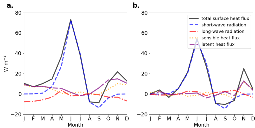
Figure 5. Anomalies (LIG-PI) of the components of the surface energy budget from a) the LIG simulation (adapted from Guarino et al., 2020b) and b) first year of LIG spin-up. For the LIG, PI, and the first year of the LIG spin-up period, the spatial average was computed from monthly data over the region from 70°N - 90°N for the simulated short-wave radiation, long-wave radiation, sensible heat flux, and latent heat flux. For the LIG and PI periods, the 200-year mean was used. The total surface heat flux anomaly (black) is the sum of these four heat budget anomalies.
