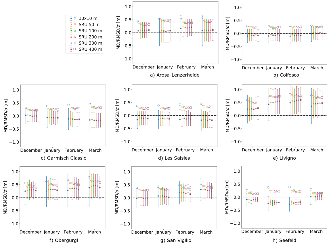
Figure 6. Overview of the root mean square deviation (RMSD, hollow symbols), mean deviation (MD, filled symbols) and standard deviation ( \sigma , extent of error bars) between simulated and GNSS measured snow depth considering all the time steps and displayed for each different SRU resolution for the entire ski resort. The presented data are analysed for the four months December, January, February and March where GNSS data were available.
