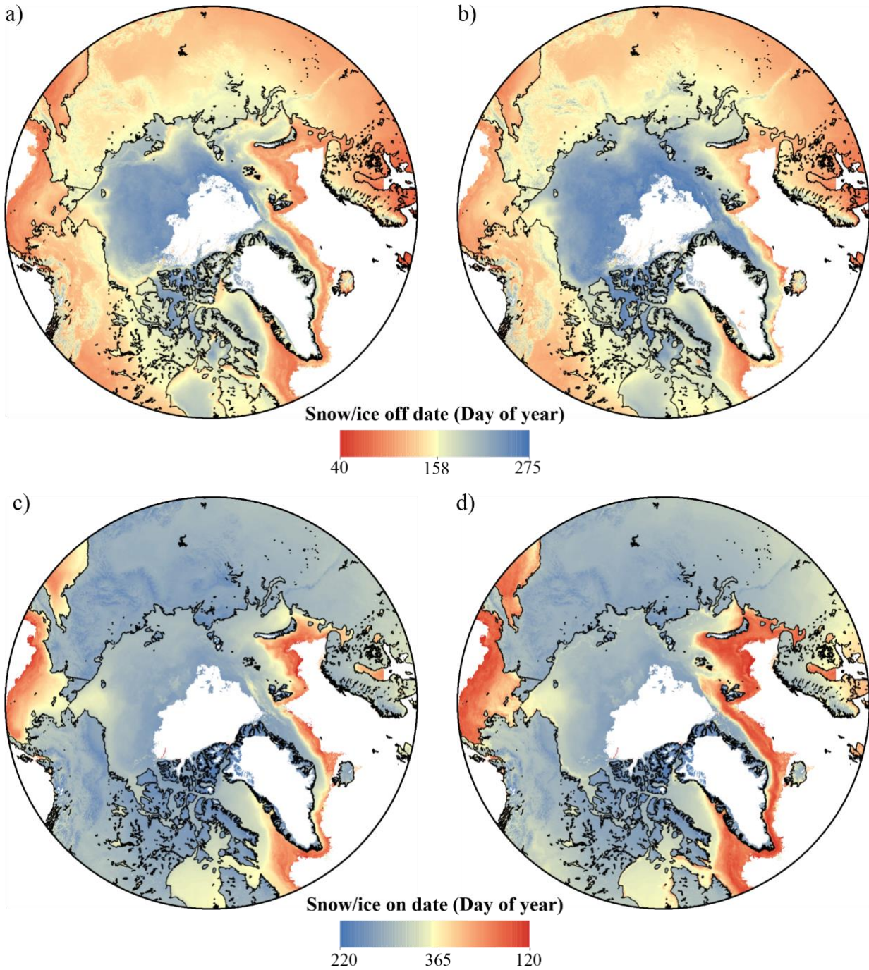
Figure 3. Mean 4 km IMS (2004 – 2019) (a) sea ice first open water (FOWs), first snow-off (first_SOFF), and lake ice first open water (FOWL), (b) sea ice water clear of ice (WCIs), final snow-off (final_SOFF), and lake ice water clear of ice (WCL), (c) sea ice freeze onset (FOs), first snow-on (first_SON), and lake ice freeze onset (FOL), and (d) sea ice continuous ice cover (CICs), final snow-on (final_SON), and lake ice continuous ice cover (CICL). White regions indicate where either no snow/ice forms, or snow/ice remains all year, in 14 or more years of the dataset.
