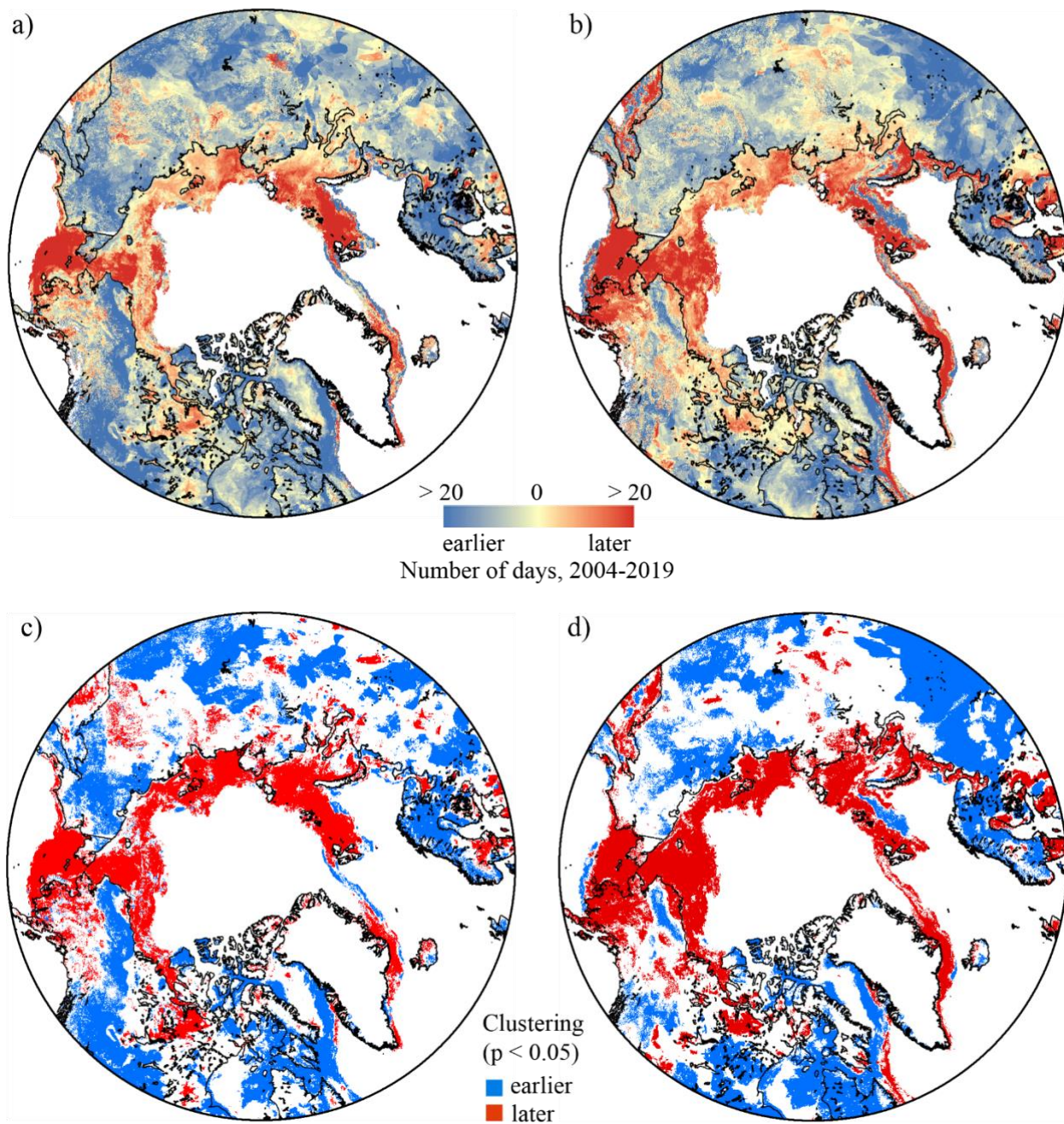
Figure 7. Trends in 4 km IMS (2004 – 2019) (a) sea ice freeze onset (FO S ), first snow-on (first_ SON ), and lake ice freeze onset (FO L ), (b) and sea ice continuous ice cover (CIC S ), final snow-on (final_ SON ), and lake ice continuous ice cover (CIC L ), (c) significant trend clusters in FO S , FO L and first_ SON , and (d) significant trend clusters in CIC S , CIC L , and final_ SON .
