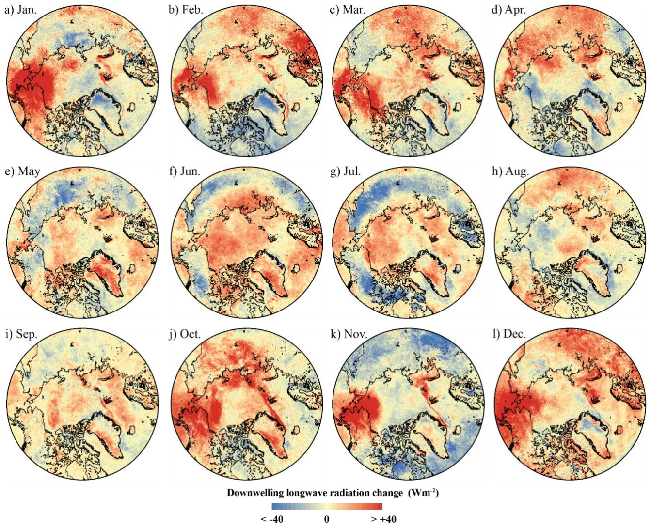
905 Figure 9: –Trends in downwelling longwave radiation 2004 – 2019 in (a) January, (b) February, (c) March, (d) April, (e) May, (f) June, (g) July, (h) August, (i) September, (j) October, (k) November, and (l) December.
