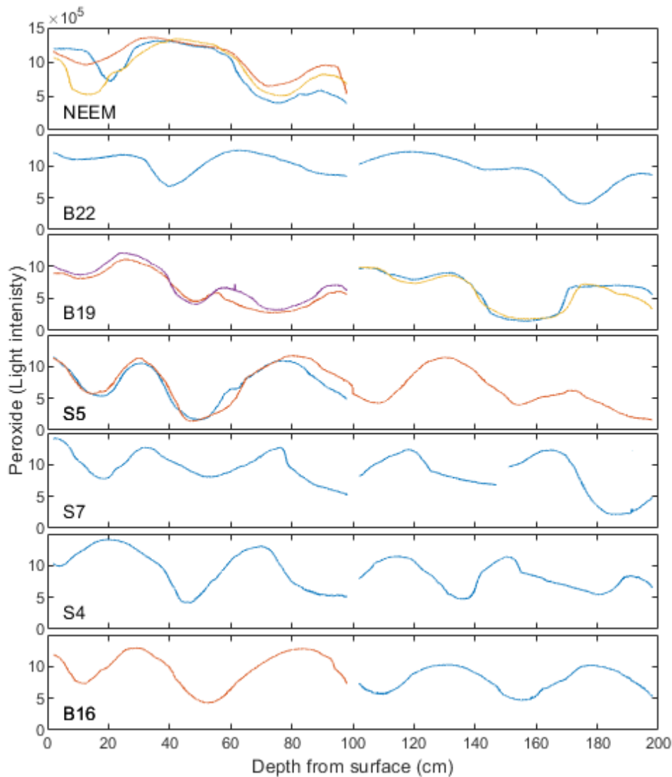
5 Figure 5: Hydrogen peroxide with depth for 7 sites in North Greenland (clockwise from North-West). For the sites NEEM, B19 and S5 several cores were retrieved. Colors indicate when multiple snow cores were collected or when the top and bottom of a pit was not measured in one run. The data are not calibrated and the y-axis is raw light intensities and thus while the level reflects the hydrogen peroxide concentration absolute values are not to be trusted.
