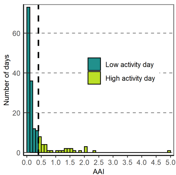
200 Figure 3: Distribution of the calculated daily AAI for days where AAI > 0. The dashed black vertical line illustrates the 0.4 AAI threshold above which days were classified as high activity days (n=34) and below which days were classified as low activity days (n=132).
