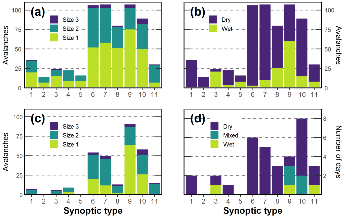
330 Figure 9. Avalanche activity by synoptic type denoted by the numeric identifier. Panel (a) displays the total number of observed avalanches of each destructive size for each synoptic type. Panel (b) shows the total number of wet and dry avalanches observed during days of each synoptic type. Panel (c) displays the total number of observed avalanches of each destructive size on high activity days of each synoptic type, and panel (d) displays the number of high activity days classified by avalanche activity wetness for each synoptic type.
