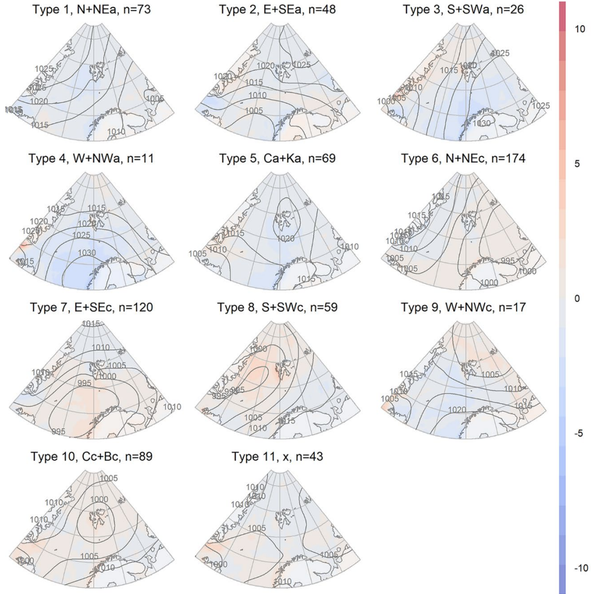
Figure A2: Composite daily accumulated precipitation anomaly by synoptic type, calculated versus mean daily accumulated precipitation conditions (Fig. B2). Composite MSLP isobars by synoptic type are included for reference.
