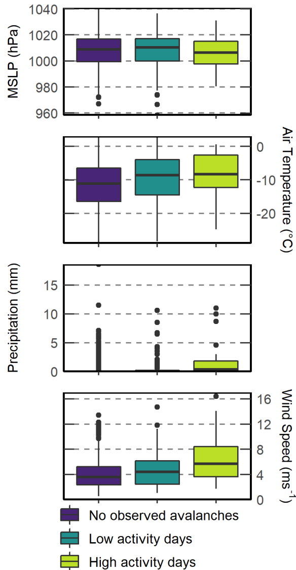
275 Figure 6: Boxplots showing the distributions for locally measured meteorological parameters by avalanche day type. Air temperature and wind speed are observed at the Gruvefjellet AWS, while precipitation and MSLP are observed at the Svalbard Airport AWS.
