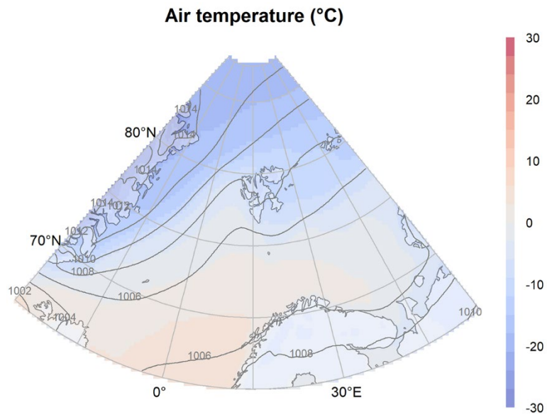
Figure B1: Mean daily air temperature composite field for all winter days (n=729) included in these analyses. This represents the mean daily air temperature conditions from which anomalies are calculated. Composite MSLP isobars for all winter days are included for reference.
