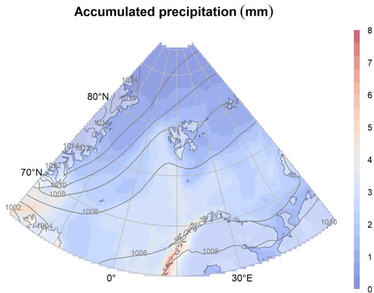
Figure B2: Mean daily accumulated precipitation composite field for all winter days (n=729) included in these analyses. This represents the mean daily accumulated precipitation conditions from which anomalies are calculated. Composite MSLP isobars for all winter days are included for reference.
