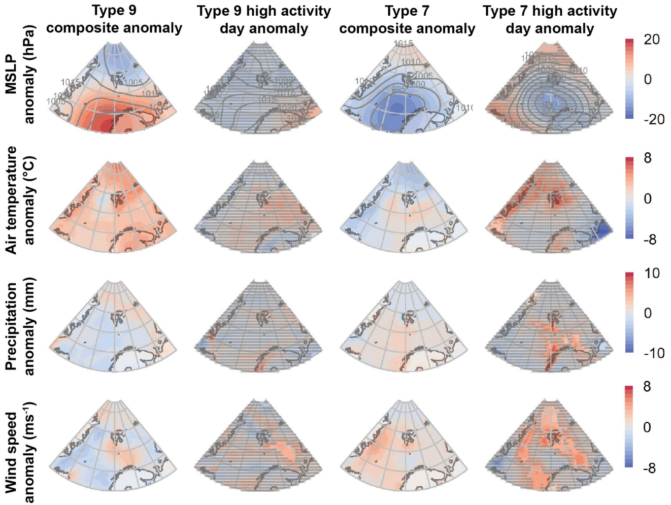
360 Figure 10: Composite anomalies for all Type 9 and Type 7 winter days vs mean winter conditions and anomalies for Type 9 and Type 7 high activity days vs Type 9 and Type 7 composites, respectively. High activity day anomalies which are not statistically significantly different from the respective synoptic type's composite are indicated with dense hatching.
