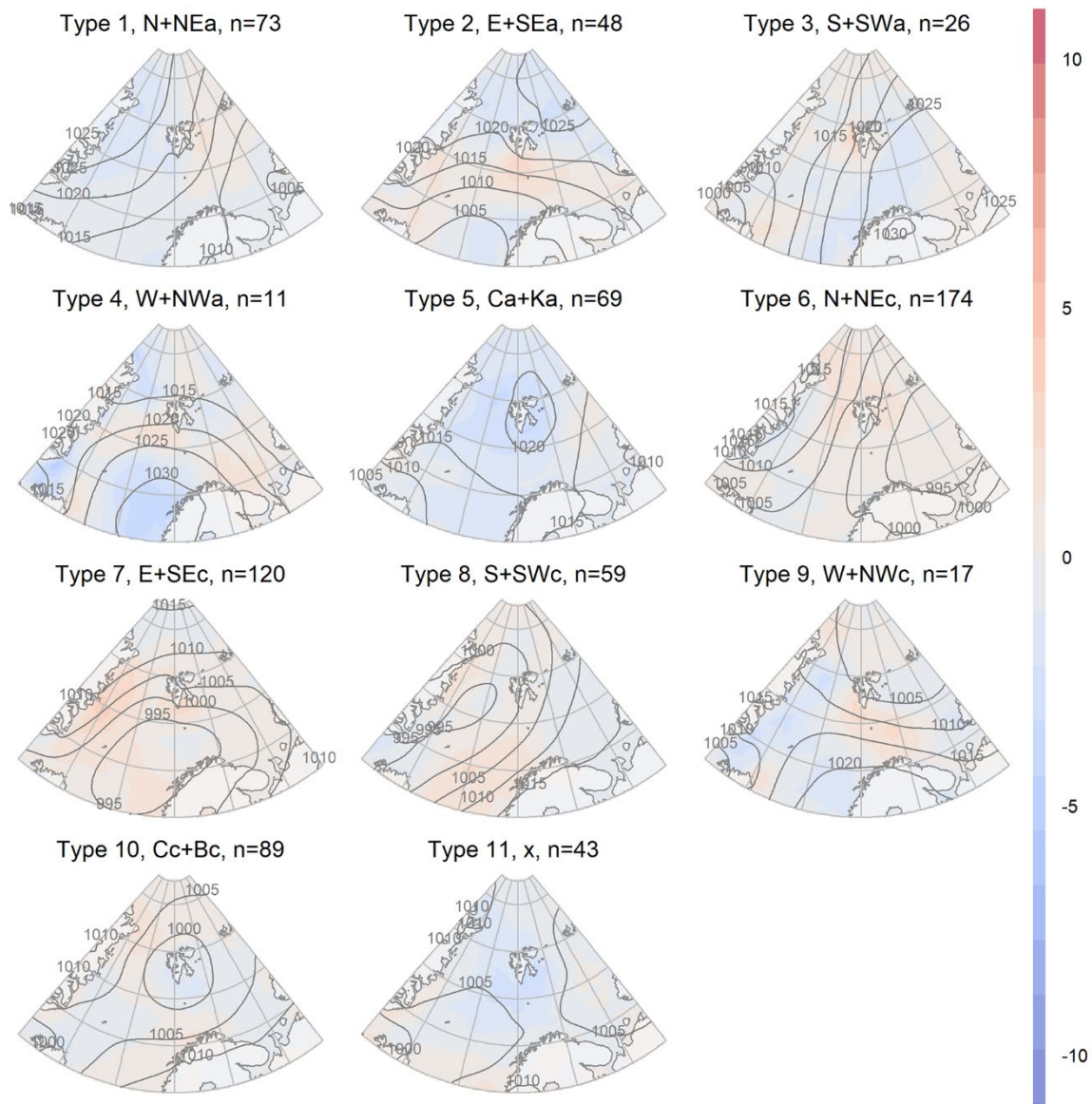
Figure A3: Composite daily mean wind speed anomaly by synoptic type, calculated versus mean daily wind speed conditions (Fig. B3). Composite MSLP isobars by synoptic type are included for reference.
