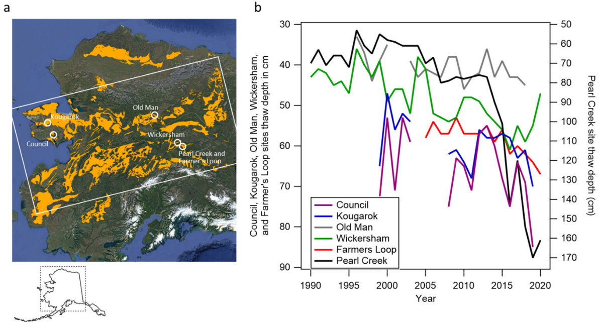
Figure 10. A) a © Google Earth map identifying yedoma type permafrost (yellow) in Alaska (Strauss et al., 2016) and locations of six central Alaska Circumpolar Active Layer Monitoring sites with records of at least 15 years. The focused field sites in this study are all near Farmer’s Loop. The white bounding box represents the 500,000 km 2 area of central Alaska across which the study measurements are extrapolated. B) active layer measurements from the six CALM sites from Interior Alaska and the Seward Peninsula. Data from CALM (2020).
