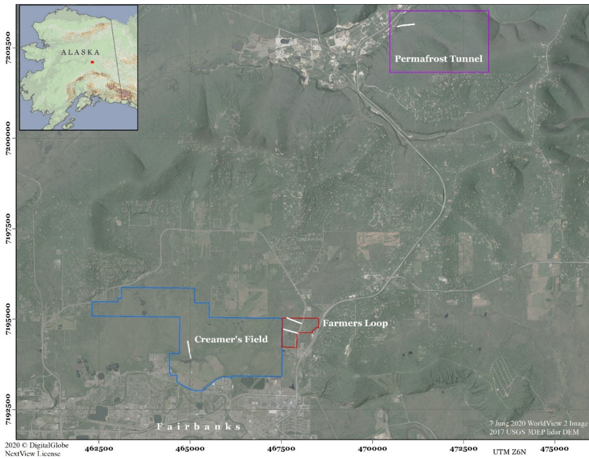
770 Figure 1. A Worldview 2 (© Digital Globe) satellite image of the area around Fairbanks, Alaska (red dot on inset map) identifying the field site sites (colored regions) and transects (white lines) in this study.
