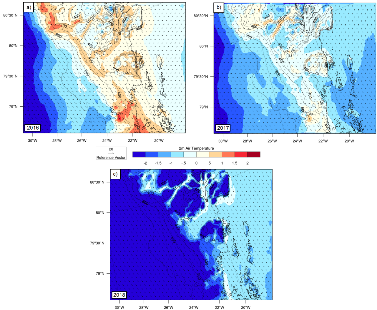
386 387 Figure 6: The monthly average 2m air temperature from PWRf runs for June 2016 (a), 2017 (b) and 2018 (c). Simulations 388 were not available for 2019. Contours are every 200 m, with labels every 400 m. Black arrows are wind vectors displaying 389 wind direction and speed, with a reference vector of 20 ms -1 provided. 390
