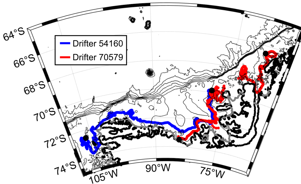
Figure 11. Drifter tracks for two drifters released as part of the LTER program and showing further support that the AACC provides a connection between the WAP and the Amundsen Sea. Drifter 54160 was released on January 1, 2007 and sent back its final position on December 24, 2007. Drifter 70579 was released on January 27, 2007 and sent back its final position on November 24, 2007; there is a gap in the data for this drifter during May 18-27 (around 74°W). Large black dots indicate the beginning and end of each drifter track.
