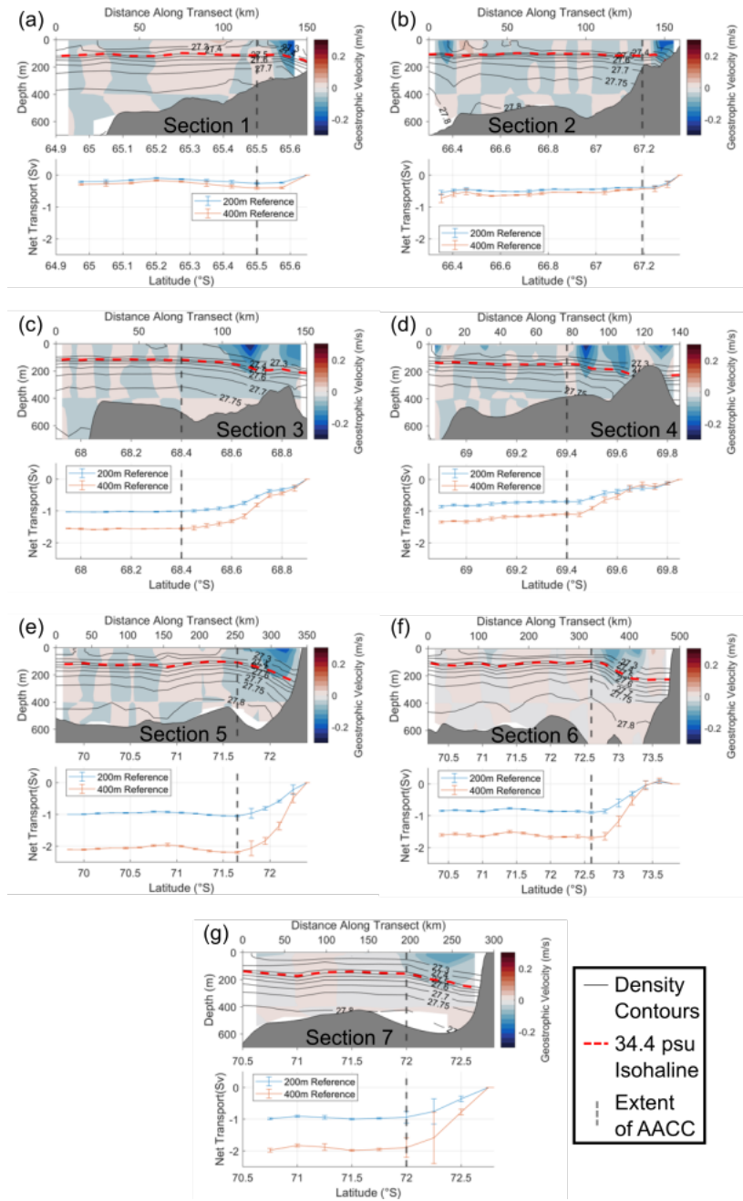
Figure 9. Geostrophic velocity (referenced to 400 m, top) and geostrophic transport (bottom) for all sections in Fig. 3. Transport values are given for both a 200 m and 400 m reference level, and transports are cumulative from the coast and calculated by integrating to the 34.4 psu isohaline. Negative (positive) values indicate transport and velocity to the west (east).
