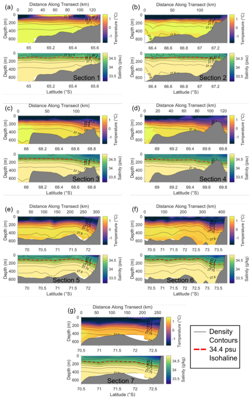
Figure 6. Vertical hydrographic sections of temperature (top) and salinity (bottom) in the upper 700 meters for each section in Fig. 3. Distance along the section is provided along the top of the temperature panels; note that sections are not of equal length.
