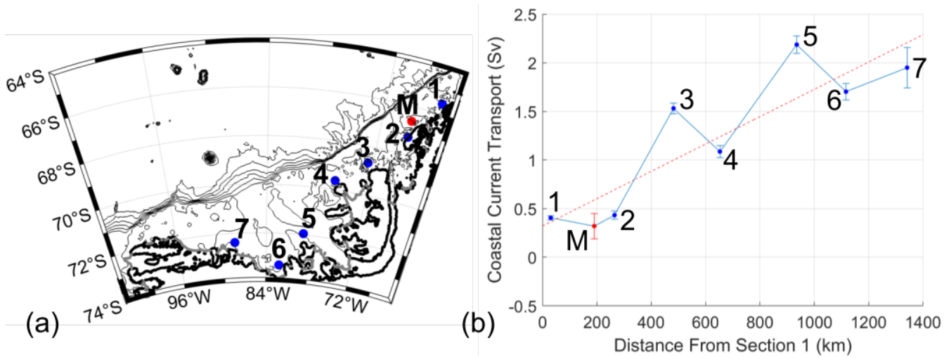
Figure 10. (a) Transport locations along the AACC from the hydrographic transects labeled the same way as in Fig. 3, and (b) the values of transport along the AACC. The transport increases as the AACC flows westward. The starting point is just north of the Moffat section, labeled with the red M, in the WAP. All of the transport values, except for Moffat et al. (2008) section, are with respect to 400 meters. The red dashed line is a trend line of 2 Sv per 1000 km. The blue dots indicate the midpoint of the AACC in each section, and the red dot is the Moffat section.
