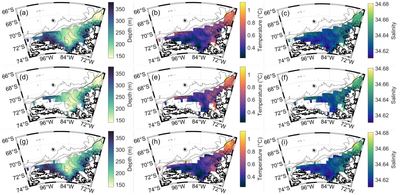
Figure A3. The distribution of properties on the the transitional layer ( 27.65 \text{ kg m}^{-3} ), divided into (top) median, (middle) winter and (bottom) summer months: (a,d,g) depth of the density layer, (b,e,h) potential temperature ( ^{\circ} \text{C} ), (c,f,i) salinity.
