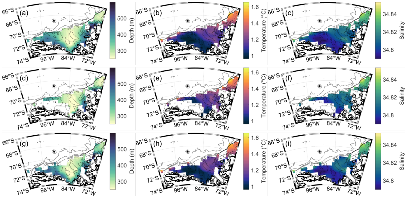
Figure A4. The distribution of properties on the the CDW layer (27.75 kg m -3 ), divided into (top) median, (middle) winter and (bottom) summer months: (a,d,g) depth of the density layer, (b,e,h) potential temperature (° C), (c,f,i) salinity.
