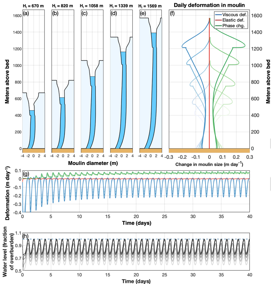
Figure 5. Contributions of viscous deformation, elastic deformation, and phase changes to moulin geometry. (a–e) Equilibrium geometries of five moulin profiles in ice of different ice thicknesses H and different distances from the terminus (same as Fig. 6o and p) averaged over the final 24 h period of a 40 d model run. (f) Vertical variation in viscous deformation (blue), elastic deformation (red), and phase change (green) contributions to moulin geometry averaged over the same 24 h period. Negative values indicate contributions to moulin closure; positive values open the moulin. Darkening shades of each color map to moulin profiles of increasing ice thickness. Closure and opening rates are greatest at the minimum daily water level (which is inferable by the lower notch in the moulin wall). (g) Time series of the components shown in panel (f) (colors the same) at the mean water level over the entire 40 d model run. The greater diurnal range in water level in moulin profiles in thick ice drives the observed larger diurnal variations in viscous deformation. (h) For reference, moulin water level as a fraction of overburden for different ice thicknesses. Lighter greys indicate thinner ice; the blue dashed line indicates where fraction of overburden = 1.
