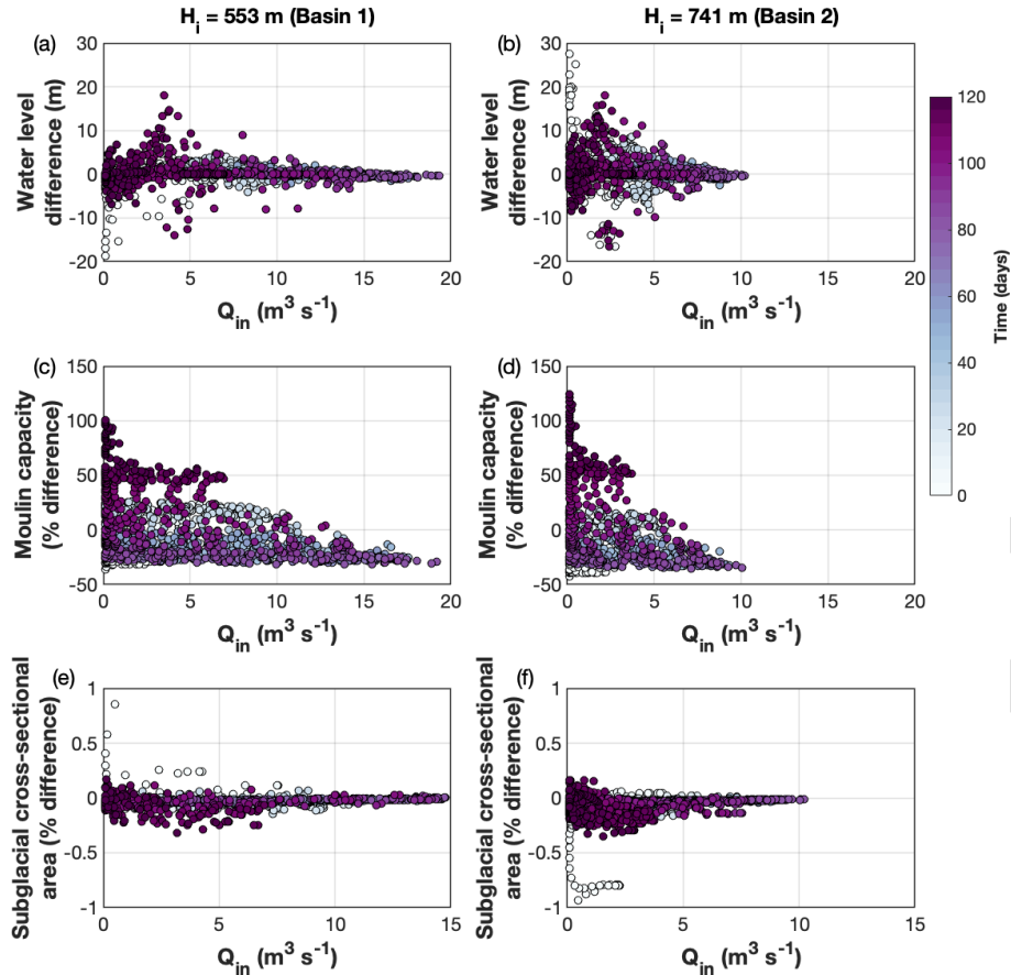
Figure 10. Difference between variable and fixed moulin geometries for Basins 1 and 2 (ice thicknesses of 553 and 741 m, respectively). The fixed moulin is a cylinder with a fixed radius of 1.6 and 1.4 m for Basins 1 and 2, respectively, which are the time-mean radii at the mean water level for the variable moulin. In all instances, the difference is calculated as (cylindrical - variable) with instances of percentage difference calculated as (cylindrical - variable) / (variable) . (a, b) Difference in moulin water level for Basin 1 and Basin 2, respectively, plotted every hour. Negative values indicate periods where the variable moulin water levels are higher than those of the fixed cylindrical moulin. (c, d) Percentage difference in moulin capacity plotted every 2 h for clarity. When values are negative, the variable moulin is larger than the fixed cylindrical moulin.
