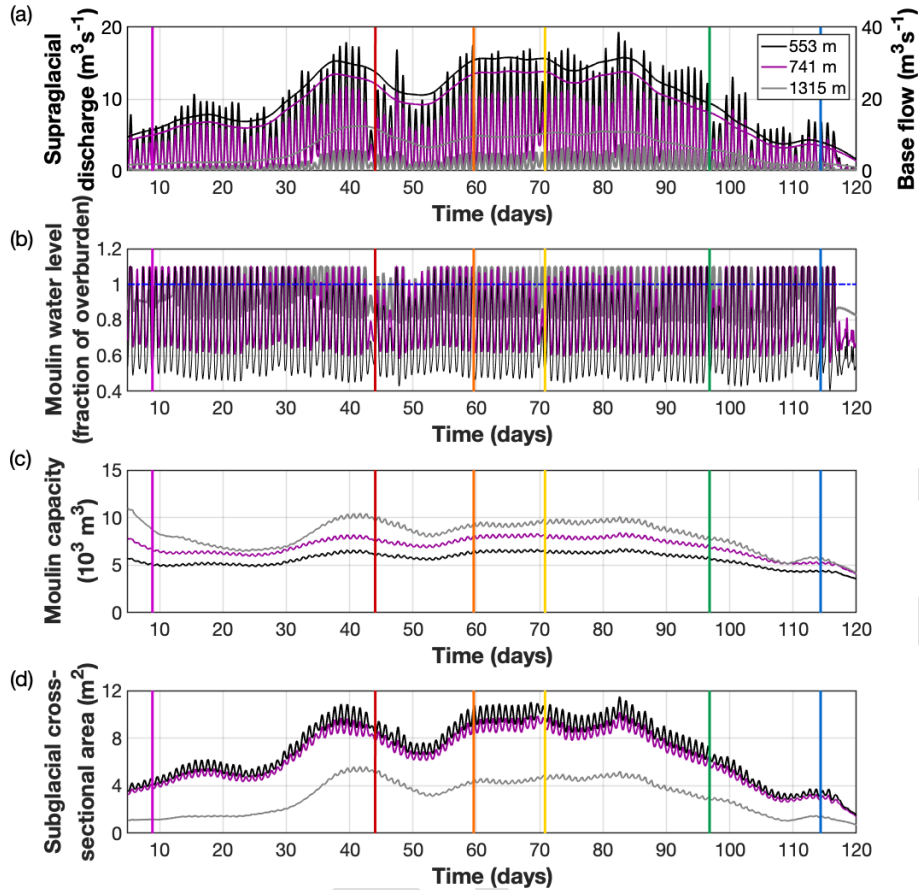
Figure 6. MouSh model runs with realistic supraglacial and ice conditions. The model runs are for a low-elevation Basin 1 ( H_i = 553 m; black lines), mid-elevation Basin 2 ( H_i = 741 m; purple lines), and high-elevation Basin 3 ( H_i = 1315 m; grey lines). (a) Supraglacial discharge into the moulin Q_{\text{in}} and prescribed base flow Q_{\text{base}} . (b) Moulin water level as a fraction of overburden. Note that the highest-elevation moulin exceeds the ice surface most days. (c) Moulin capacity, or the total moulin volume. (d) Subglacial channel cross-sectional area. Colored vertical lines indicate times in Fig. 7. Note x axes start on day 5.
