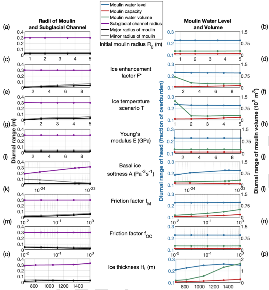
Figure 4. Diurnal variations in moulin sizes in 40 d parameter sensitivity runs. Shown are the sensitivity of diurnal variation in moulin size and water storage metrics to initial condition for moulin radius (a, b), enhancement factor for englacial ice (c, d), ice temperature scenario from coldest to warmest ice (e, f), Young’s modulus (g, h), softness of basal ice (i, j), friction factor for water flow beneath the water line (k, l), friction factor for water flow above the water line (m, n), and ice thickness (o, p). The left column shows diurnal variations in moulin radii (black and grey) at the equilibrium water level and the subglacial channel radius (purple) in the final 24 h period of the 40 d model run. The right column shows the diurnal variation in water level (blue), moulin capacity (red), and volume of water in the moulin (green) within the same 24 h period. Note the right y-axis difference in panel (p).
