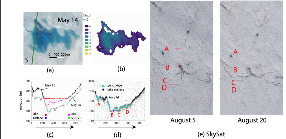
Figure 10. ICESat-2 RGT 727 over Lake Julian. (a) Sentinel-2 based imagery acquired on May 14 th 2019 with ICESat-2 RGT 727 overlaid (occurring on May 15 th , 2019 and August 14 th , 2019) overlapping in green. Operation IceBridge overpass on May 15 th , 2019 is directly coincident with the ICESat-2 line. (b) Lake depth derived from Watta (Panel c) and Sentinel-2 imagery (Panel a) based depth. (c) Watta calculated from ICESat-2 on May 15 th and Aug 14 th . (d) Watta-calculated surface features over photon cloud on Aug 14 th . Points A-D discussed in text (e) Points A-D shown over Planet SkySat imagery collected on August 5 th and August 20 th .
