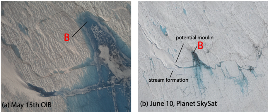
480 Figure 9. Mechanisms of lake drainage over Lake Julian. (a) CAMBOT imagery from Operation IceBridge flight on May 15 th , 2019 (30cm resolution). (b) SkySat imagery (~1m resolution) on June 10 th after large-scale drainage
