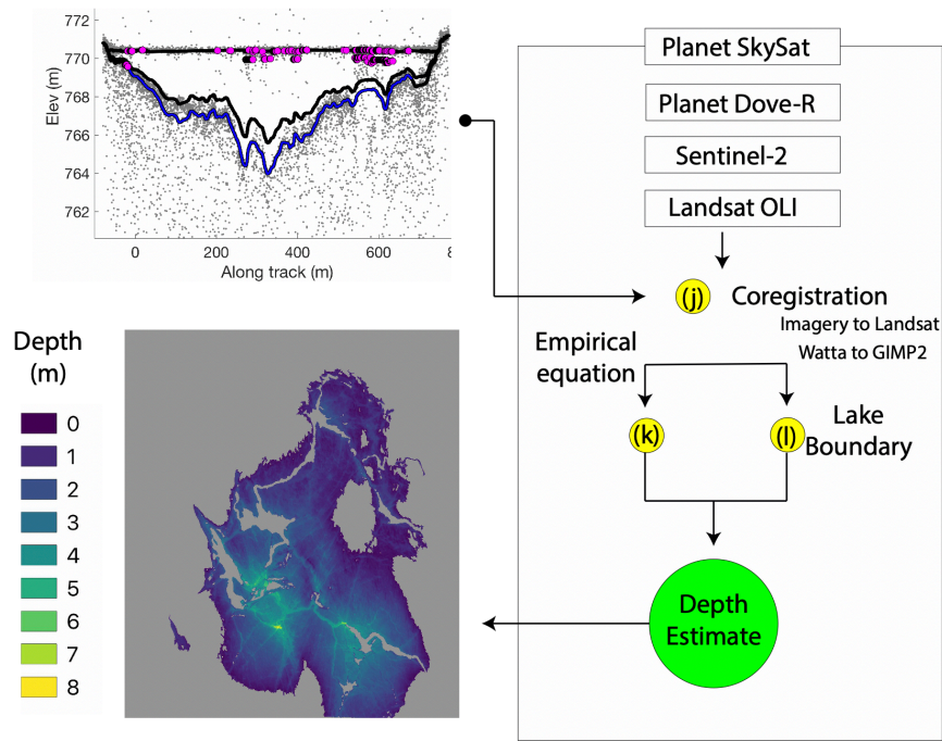
295 Figure 3. Diagram of imagery processing steps accepting Watta outputs as input (top left) and producing lake depth estimates (bottom left). Watta lake depth profile shown is for Lake Ayse using RGT 841 on May 23 rd and Planet SkySat imagery on May 22 nd .
