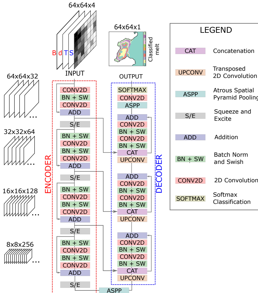
Figure B1. Schematic for the segmentation network used in this study. An input 64 \times 64 \times 4 image goes through layers of 2D convolutions, batch normalisations and swish layers through the decoding and encoding branches. Once trained on NEMO results, the final output is a segmented image consisting of melt rate labels that can then be converted into a melt rate field using the DAE network.
