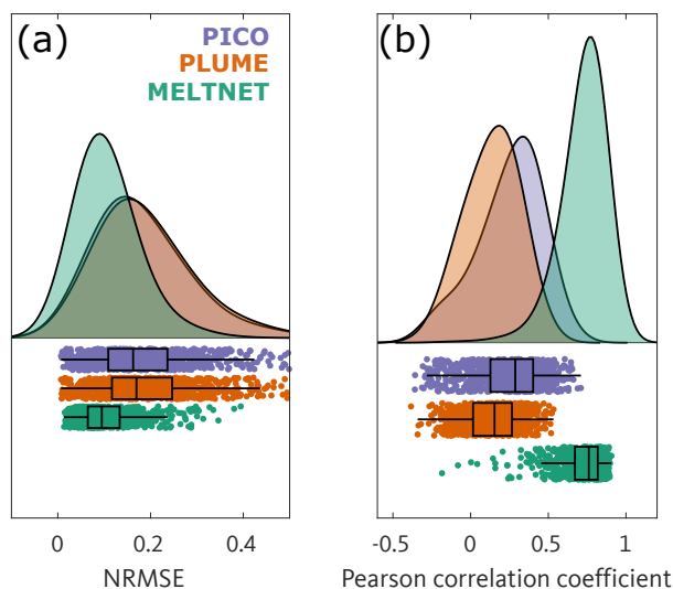
Figure 4. Distributions of NRMSE (panel a) and Pearson correlation coefficient (panel b) for the three different melt rate parameterisations: PICO (violet), PLUME (orange) and MELTNET (green). The lower section of each panel shows each individual score from the entire test set, overlain with a boxplot. The box represents the interquartile range of scores and the vertical line through the box is the median. The upper section of each panel presents the same information as probability density plots. Note lower NRMSE and higher correlation coefficient mean a better fit to the groundtruth NEMO melt rates.
