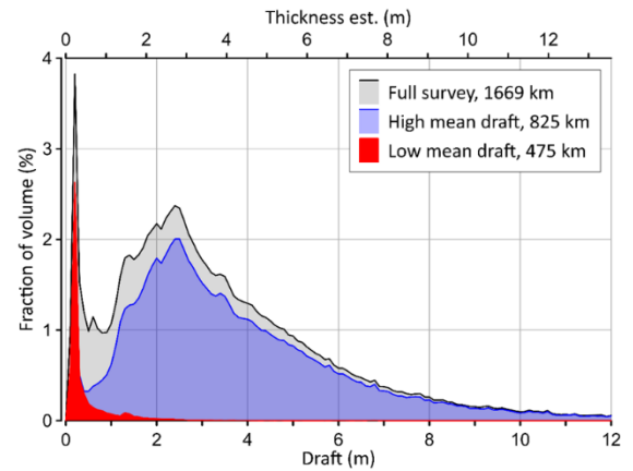
Figure 7. Fraction of ice volume versus draft. The curves represent all data, data from 33 25-km segments with mean draft over 2.5 m and data from 19 with mean draft under 1.5 m. Thickness on the top axis is estimated as 1.13x draft..
