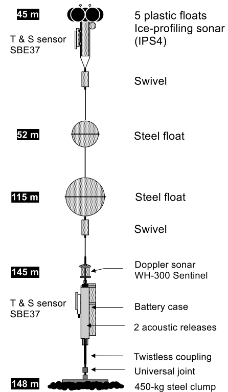
Figure 3. Mooring used to support sonar in Penny Strait. The twistless coupling enables measurement of ice-drift direction.
