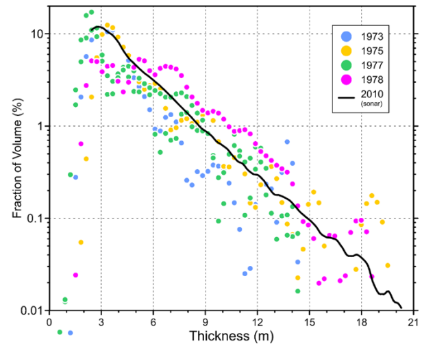
Figure 13. Distribution of pack-ice volume over ice thickness in Penny Strait comparing recent data with surveys during the 1970s. The 2009 data have been adjusted to late winter 2010, as explained in the text.
