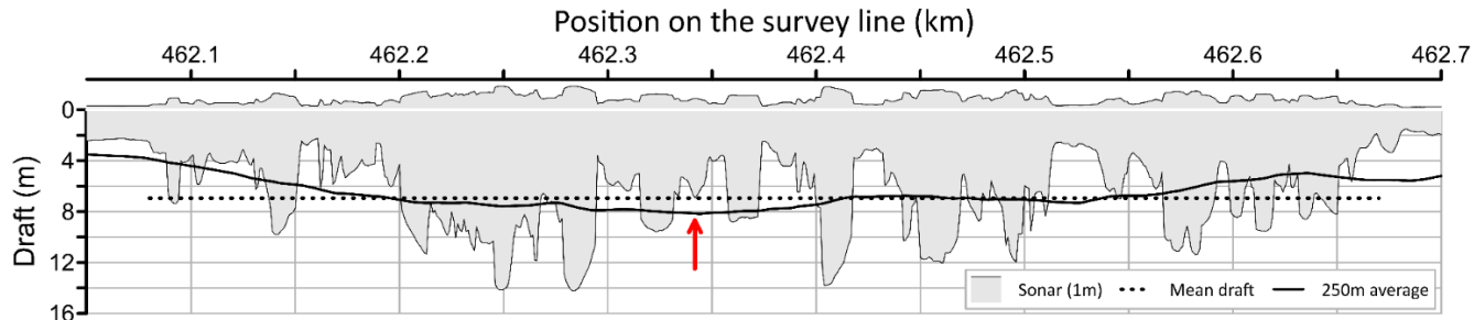
Figure 17. A 650-m section of a floe with 6.95m average draft showing the difference between conventional ridge keels of 25-m scale in the original sonar record and the identified "keel" (arrow) in the 250-m averaged draft. Plotted freeboard is simply a notional scaled version of the floe’s draft.
