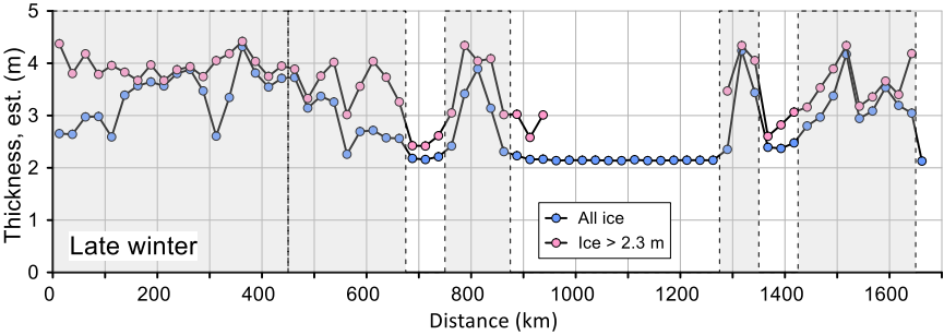
Figure 11. Average ice thickness for 25-km segments of the track line at the end of the 2009-10 winter, estimated by forcing ice growth with monthly climatological data for air temperature and snow depth, with the assumption that no new leads or ridges formed during the winter. Shading denotes intervals with appreciable multi-year ice.
