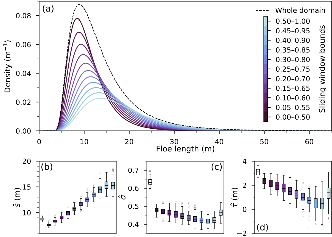
Figure 6. (a) FSDs, estimated by kernel density estimation fitted to lognormal distributions , in the whole domain and various sub-domains, as described in the text . The area under the partial FSDs are scaled by the number of observations, so that summing the first and the last windows, covering non-overlapping halves of the domain, yields the whole domain FSD. The effective number of floes, relative to the total number of floes in the domain, decreases steadily from 0.61 0.64 to 0.39 0.36 . Densities averaged over 500 realisations. (b–d) Variation of the estimated parameters among the 500 realisations . In each panel, the leftmost, white box corresponds to the whole domain; the coloured boxes follow the colour bar in panel (a).
