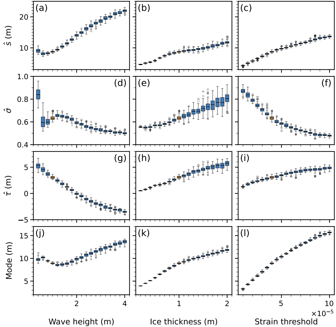
Figure 7. (a-i) Estimated Box-and-whisker plots of the estimated lognormal parameters for different model configurations. (j-l) Distribution mode Box-and-whisker plots of the modal floe size derived from the estimated parameters (Eq. (27)). Mean values with one standard deviation error bars The plots show the variation across 500 realisations. The reference configuration is highlighted with a contrasting colour, where the size of the boxes allow .
