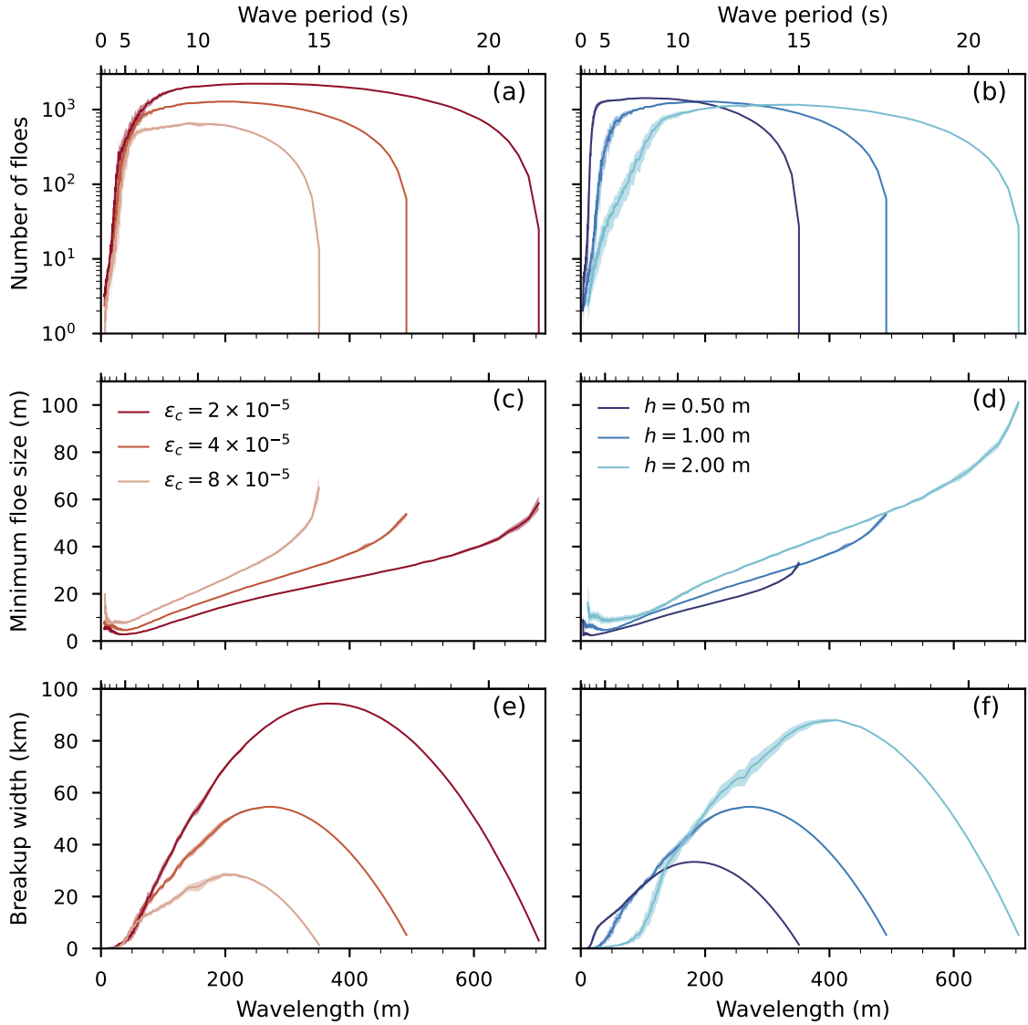
Figure 4. Various metrics at the end of a simulation. (a) Number of floes at the end of a simulation for different \epsilon_c . (b) Same as (a) but for different h . (c) Minimum floe size in the sample for different \epsilon_c . (d) Same as (c) but for different h . (e) Breakup width for different \epsilon_c . (f) Same as (e) but for different h . The breakup width is defined as the cumulated length of the broken off floes. In (a,c,e) h = 1 m; in (b,d,f) \epsilon_c = 4 \times 10^{-5} ; T = 8 s, a = 50 cm for all panels. The wavelength axis corresponds to the open-water propagating wavelength at a given T . Darker hues denote weaker ice (higher strain threshold, lower thickness) and lighter hues denote stronger ice. The plotted lines are ensemble average, the shaded areas indicate one standard deviation.
