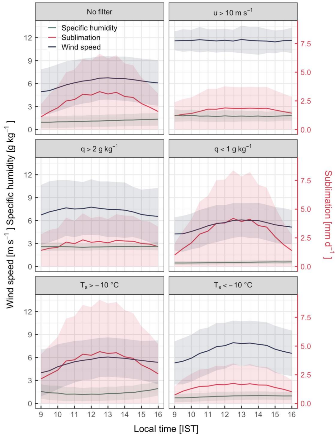
Figure 12. Half-hourly daytime (09:00-16:00) records of sublimation (red), wind speed (blue) and specific humidity (green) at the AWS-M for different clusters: no filter, u > 10 \text{ m sec}^{-1} , q > 2 \text{ g kg}^{-1} , < 1 \text{ g kg}^{-1} , T_s > -10^\circ\text{C} and T_s < -10^\circ\text{C} . Data period: DJFMA, 2009-2020. Number of data-points n=30257, 2347, 12295, 9762, 10552 and 12734 for no filter, u > 10 \text{ m sec}^{-1} , q > 2 \text{ g kg}^{-1} , < 1 \text{ g kg}^{-1} , T_s > -10^\circ\text{C} and T_s < -10^\circ\text{C} , respectively.
