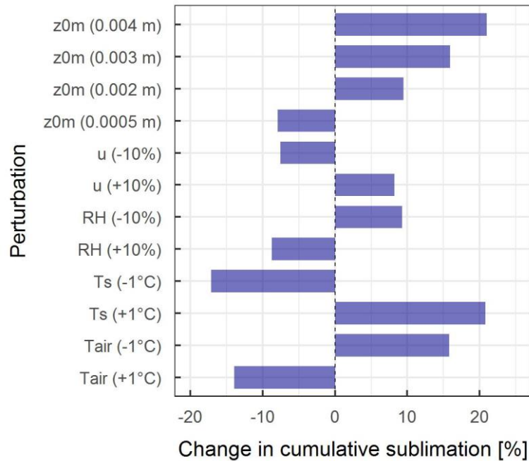
575 Figure 14. Calculated change in mean cumulative sublimation after applying perturbations to T_{air} ( \pm 1^\circ\text{C} ), T_s ( \pm 1^\circ\text{C} ), u ( \pm 10\% ), RH ( \pm 10\% ), snow z_{0m} (0.0005 m, 0.002 m, 0.003 m, and 0.004 m).
