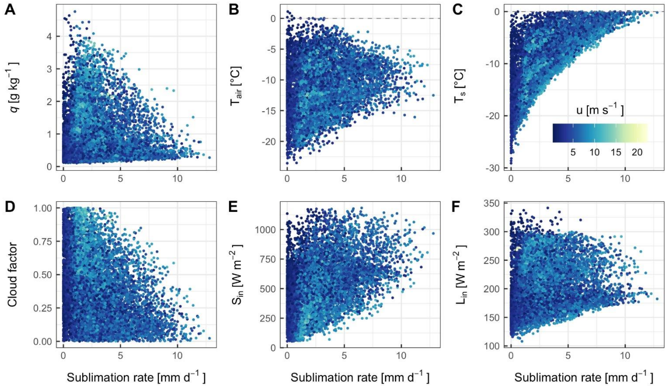
Figure 13. Scatter plot of u , q , T_{air} , T_s , CF , S_{in} and L_{in} against sublimation rate at the AWS-M. The colour of the data points refers to the measured wind speed ( u ). Total n = 14088 half-hourly data points between 09:00 and 16:00 IST for DJFMA (2009-2020).
