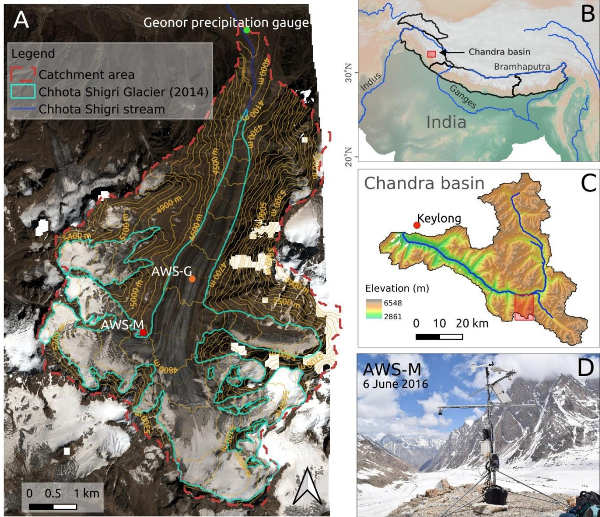
Figure 1. (A) Chhota Shigri Glacier catchment showing the location of the AWS-M (red dot; middle ablation zone) and AWS-G (orange dot; middle ablation zone) and Geonor T-200B automatic precipitation gauge (green dot). Glacier outline was derived using the 2014 Pléiades image (Azam et al., 2016). The background is the Pléiades ortho-image of 12 September 2020 (copyright CNES 2020, distribution Airbus D&S). (B) Location of the Chhota Shigri Glacier region in the western Himalaya. (C) Map of the Chandra Basin, with Chhota Shigri catchment marked (red rectangle). Elevation based on the Shuttle Radar Topographic Mission (SRTM) Digital Elevation Model (DEM) obtained from the United States Geological Survey (USGS). (D) Photo of the AWS-M on the lateral moraine (Photo credit: A Mandal).
