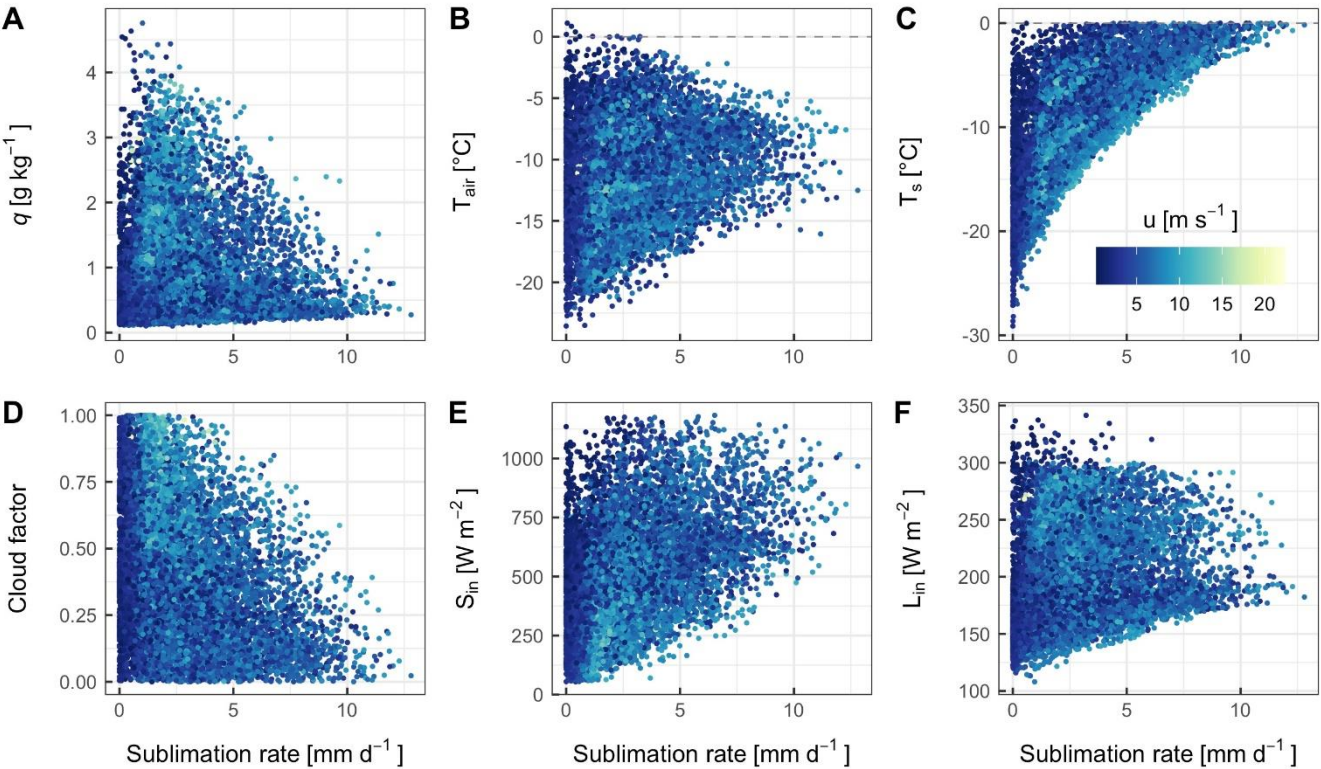
Figure 13. Scatter plot of u, q, T_{air}, T_s, CF, S_{in} and L_{in} against sublimation rate at the AWS-M. The colour of the data points refers to the measured wind speed ( u ). Total n = 14088 half-hourly data points between 09:00 and 16:00 IST for DJFMA (2009-2020).
