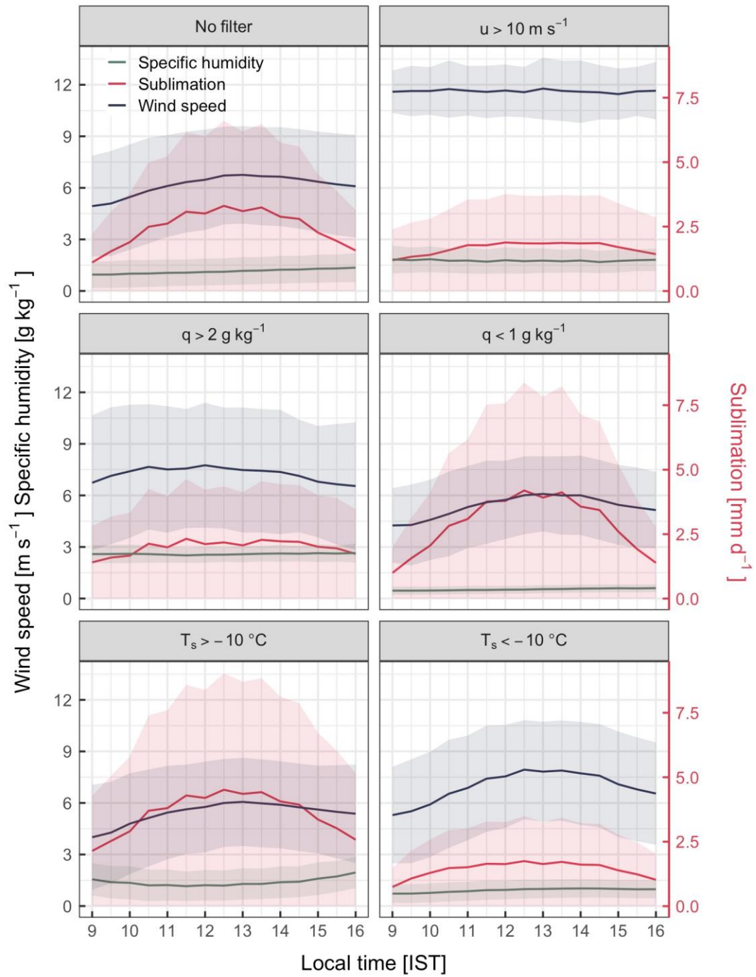
485 Figure 12. Half-hourly daytime (09:00-16:00) records of sublimation (red), wind speed (blue) and specific humidity (green) at the AWS-M for different clusters: no filter, u > 10 \text{ m sec}^{-1} , q > 2 \text{ g kg}^{-1} , < 1 \text{ g kg}^{-1} , T_s > -10^\circ\text{C} and T_s < -10^\circ\text{C} .
