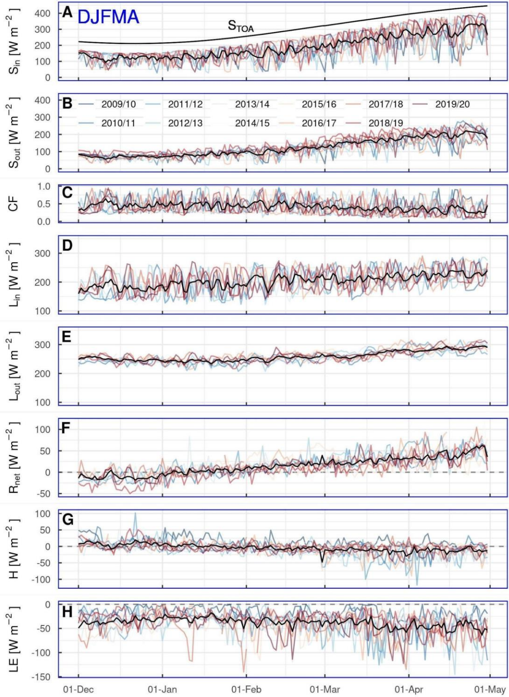
Figure 5 (revised manuscript). The daily mean of short-wave radiation at the top of the atmosphere ( S_{\text{TOA}} ), short-wave incoming ( S_{\text{in}} ) and outgoing ( S_{\text{out}} ), cloud factor ( CF ), long-wave incoming ( L_{\text{in}} ) and outgoing ( L_{\text{out}} ), net radiation ( R_{\text{net}} ), turbulent sensible ( H ) and latent ( LE ) heat fluxes at the AWS-M for DJFMA, 2009-2020. L_{\text{in}} and R_{\text{net}} start from 1 December 2010. The black line highlights the mean of 2009-2020.
