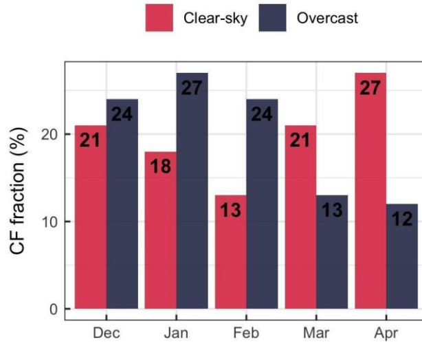
Figure 8 (in revised manuscript). Monthly fraction of clear-sky ( CF \leq 0.2 ) and overcast ( CF \geq 0.8 ) conditions at the AWS-M. Fraction percentage is calculated from n = 5810 clear-sky and n = 2381 overcast observations from total n = 23903 half-hourly values between 09:00 and 16:00 IST (DJFMA, 2009-2020).
