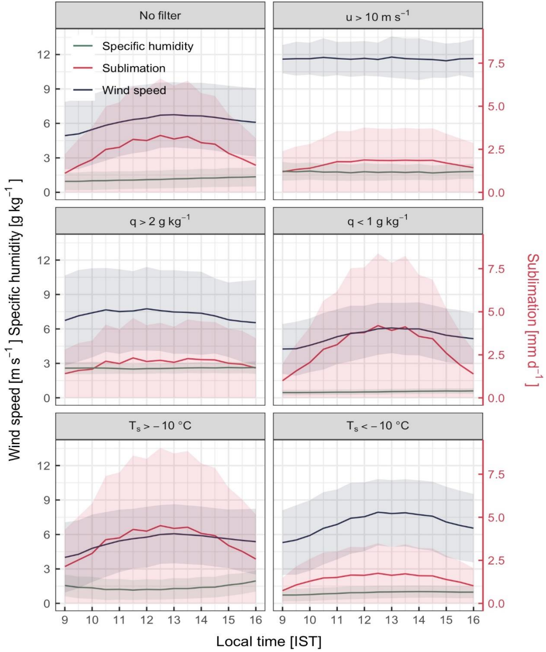
Figure 12 (in revised manuscript). Half-hourly daytime (09:00-16:00) records of sublimation (red), wind speed (blue) and specific humidity (green) at the AWS-M for different clusters: no filter, u > 10 \text{ m sec}^{-1} , q > 2 \text{ g kg}^{-1} , < 1 \text{ g kg}^{-1} , T_s > -10^\circ\text{C} and T_s < -10^\circ\text{C} . Data period: DJFMA, 2009-2020. Number of data-points n=30257 , 2347, 12295, 9762, 10552 and 12734 for no filter, u > 10 \text{ m sec}^{-1} , q > 2 \text{ g kg}^{-1} , < 1 \text{ g kg}^{-1} , T_s > -10^\circ\text{C} and T_s < -10^\circ\text{C} , respectively.
