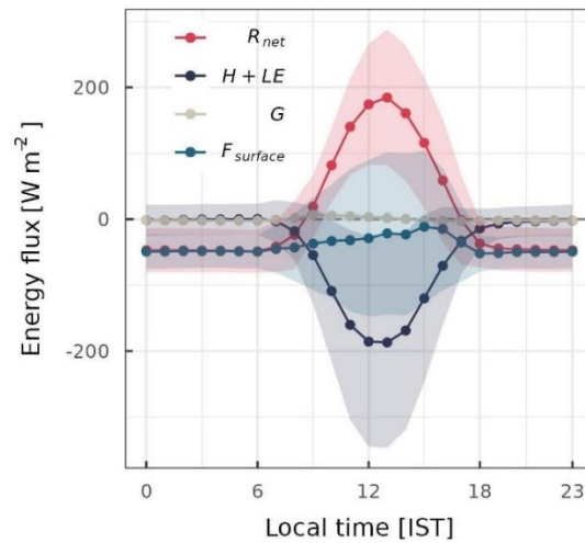
Figure R2. Mean diurnal cycle of G (following You et al., 2014 and Luce and Tarboton, 2010) at the AWS-M for DJFMA (2009-2020) along with R_{net} , H + LE , and F_{surface} .
