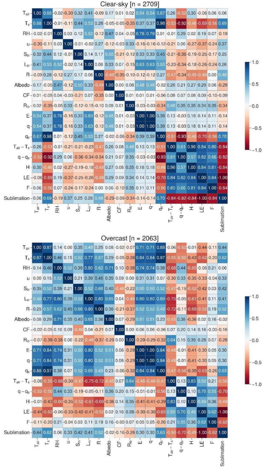
Figure 11 (in revised manuscript). Pearson's correlation coefficient ( r ) matrix of various meteorological and SEB components at the AWS-M in clear-sky and overcast conditions between 09:00 and 16:00 IST, 2009-2020. Number ( n ) of half-hourly data points are shown on top of the panels.
