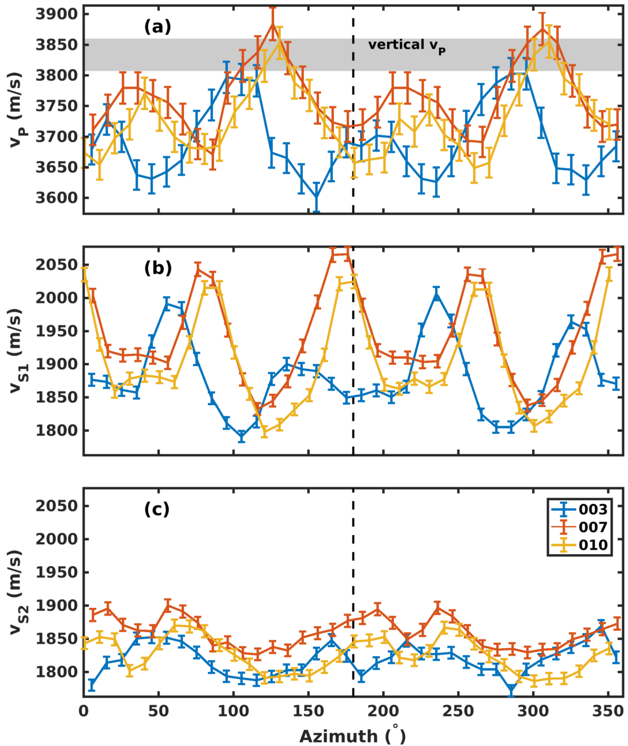
Figure 5. Ultrasonic multi-azimuth velocities for different core sections relative to the macroscopic glacier flow direction (0°). (a) P-wave velocity v_P . The gray-shaded box shows the range of measured vertical ultrasonic v_P . (b) Fast S-wave velocity v_{S1} . (c) Slow S-wave velocity v_{S2} .
