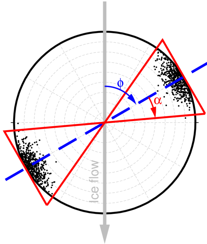
Figure 6. Upper-hemisphere stereographic projection c-axis orientations of an example Horizontal-Cluster-CPO model with illustration of model parameters: Cluster orientation \varphi and opening angle \alpha .
