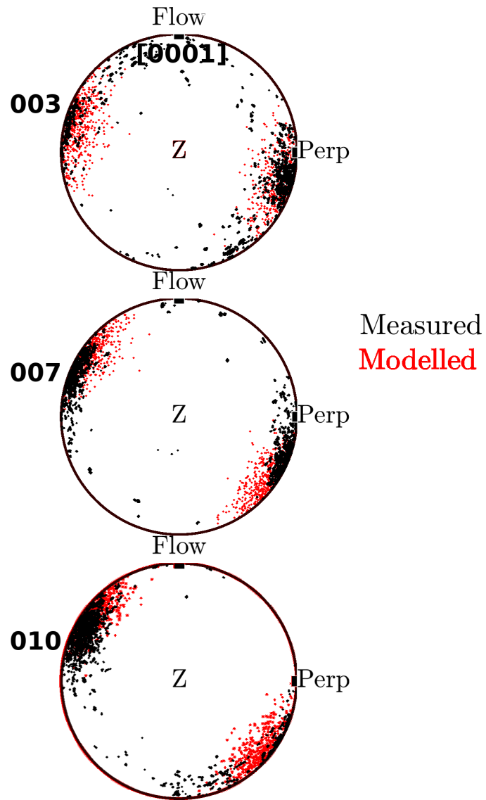
Figure 11. Measured (black) and modelled (red) CPO geometries. c-axis orientations in an upper-hemisphere stereographic projection are shown. The VSP profile orientations of the “Flow” and “Perp” profiles are labelled. Top: sample 003, middle: sample 007, bottom: sample 010.
