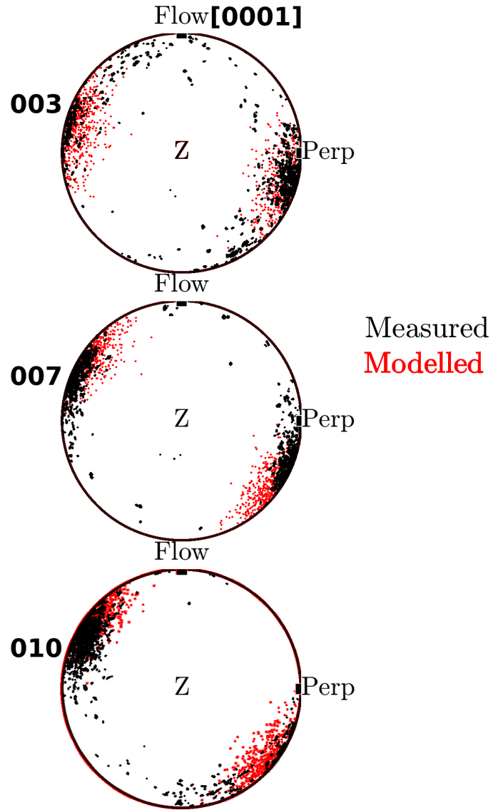
Figure 11. Measured (black) and modelled (red) CPO geometries. The VSP profile orientations of the “Flow” and “Perp” profiles are labelled. Top : sample 003, middle : sample 007, bottom : sample 010.
