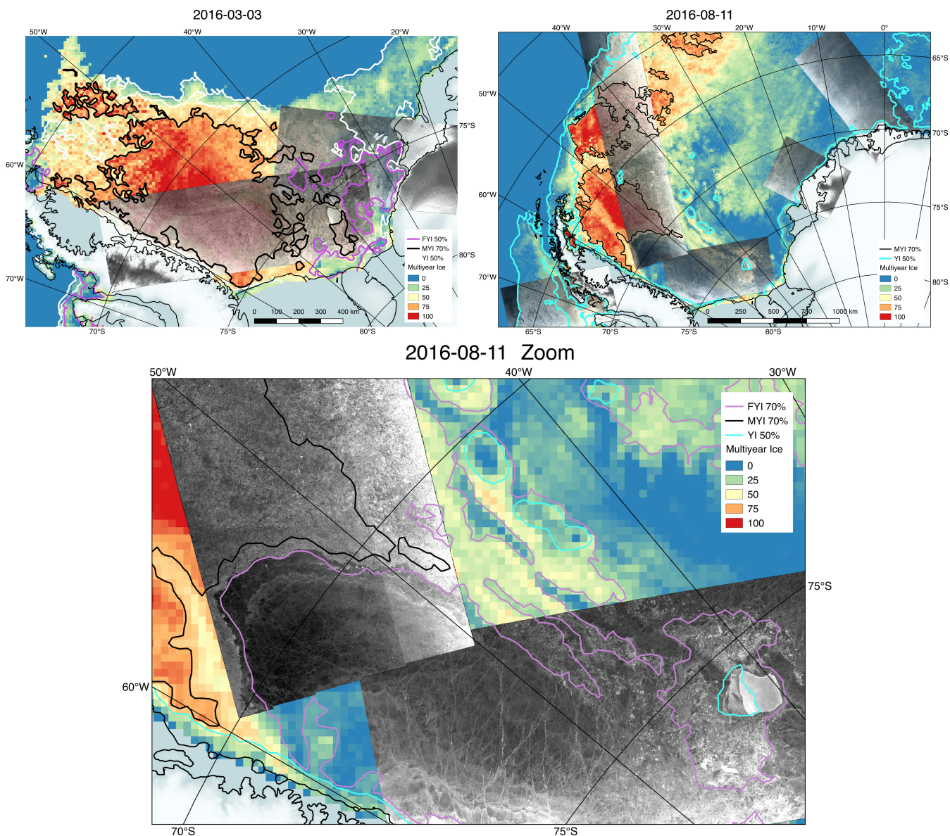
Figure 3. Sentinel-1 SAR image (grey shade) acquired on 3 March and 11 August, 2016, overlaid on MYI concentration (colour scale) of the same days from ECICE. At the top an overview of the Weddell and adjacent seas for the two days is shown. the bottom map shows a zoom in to an area is the inner (Southeastern) Weddell Sea, bordering the Antarctic Peninsula (lower left corner of the Figure). Dominant ice type from ECICE are indicated by contour lines. The MYI color legend shows only the most important colours for multiples of 25% concentration.
