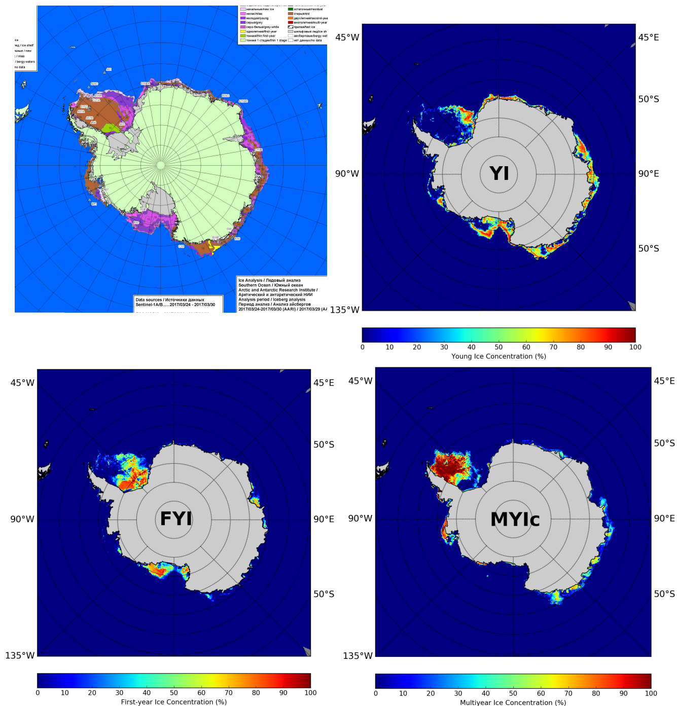
Figure 4. Top left: Stage of Development (SoD) chart by AARI, 30 Mar, 2017; top right: YI concentration (ECICE), bottom left, FYI concentration (ECICE); bottom right: corrected MYI concentration (MYIc, ECICE and correction schemes). In the SoD chart, purple shades are YI (see colour legend in the appendix, Table B1), yellow and green shades are FYI, and brown and orange/red shades are MYI.
