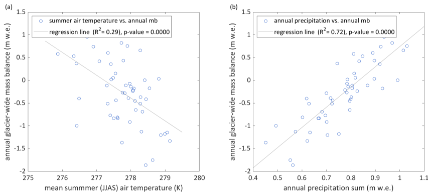
Figure 15. Climate variables at the station location (3837 m a.s.l.) versus modelled mass balance: Mean summer air temperature versus annual mass balance (a) and annual precipitation sums versus mean annual mass balance. figure axes corrected and moved to supplement
