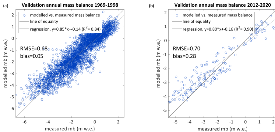
Figure 6. Model validation: Measured versus modelled annual surface mass balance for an independent set of point measurements from 1968/1969-1997/1998 (a) and from 2011/2012-2019/2020 (b). (updated axis)
