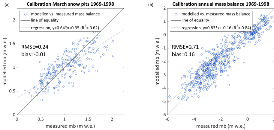
Figure 14. Model parameter calibration: Measured versus modelled surface mass balance for end of March (a) and September (b) for point measurements which are used for model calibration (1968/1969-1997/1998). The final calibration is shown. The bias between modelled and measured w.e. for snow pit measurements at the end of March (a) is minimised by optimising the precipitation correction factor. The bias between modelled and measured September mass balance measurements is optimised by tuning the albedo of ice. figure axes corrected and moved to supplement
