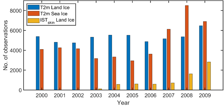
Figure 1: Total number of daily averaged in situ observations of T2m and IST_{skin} over Arctic land ice and sea ice per year covering the period 2000-2009.
