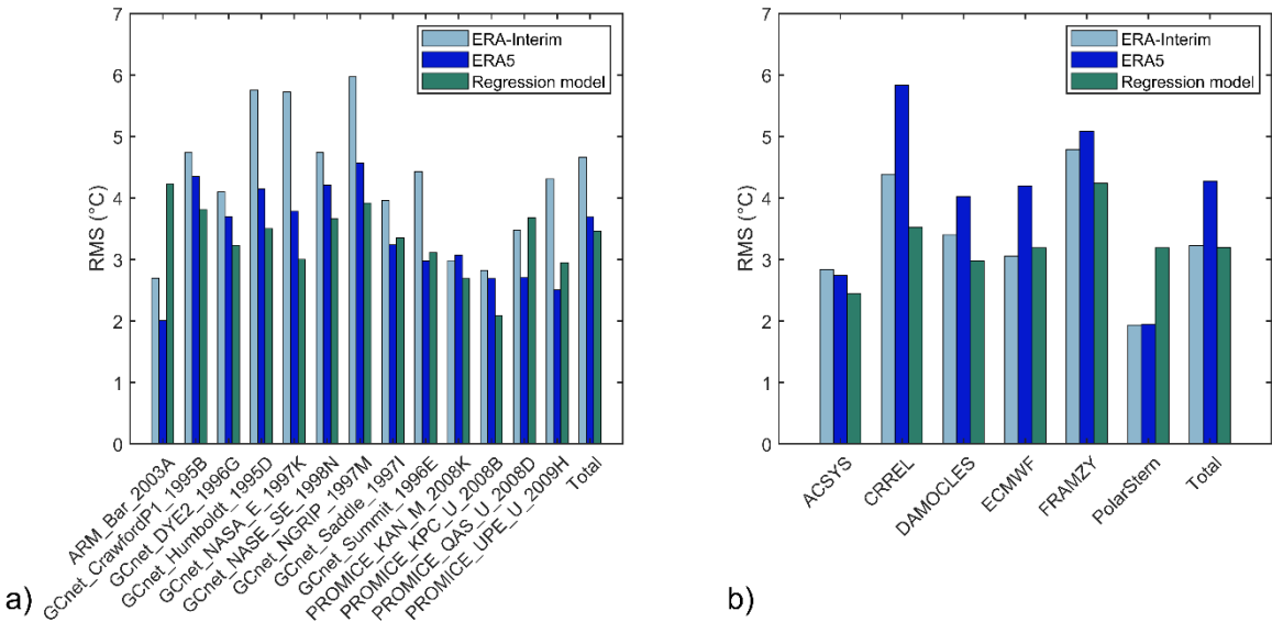
Figure 12: Root mean square (RMS) differences calculated for the (a) land ice sites and (b) sea ice sites using T2m from ERA-Interim, ERA5 and the regression model, respectively. Only buoys with more than 200 observations are included. The last two bars listed as “total” are the RMS obtained by using all validation data.
