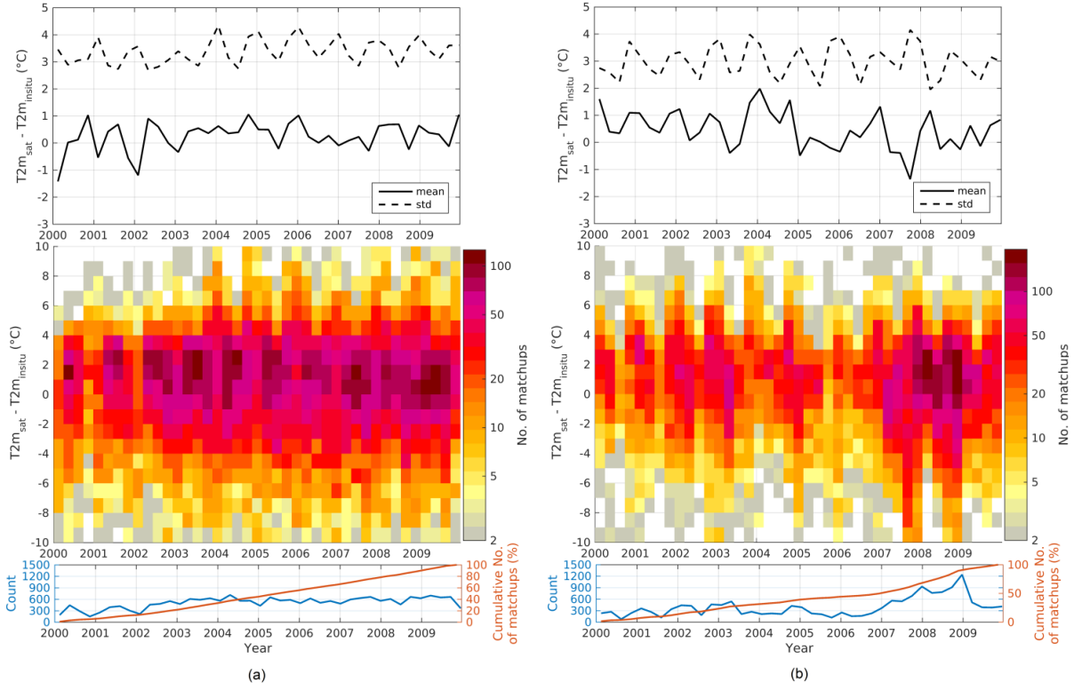
Figure 8: Estimated T2m minus observed T2m (bin size of 1°C) for the full time period (bin size of 90 days) for (a) land ice and (b) sea ice. The dashed lines are standard deviations while the solid lines are bias in the upper figures. The surface plots in the middle figures show the number of matchups in each bin, while the bottom plots show the number of matchups (blue) and the cumulative percentage of matchups (red) in each time bin.
