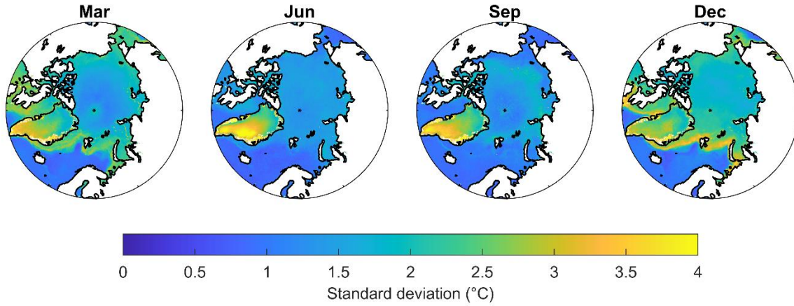
Figure 4: Standard deviations (°C) of daily satellite surface temperature observations for March, June, September and December of each year averaged for the years 2000-2009.
