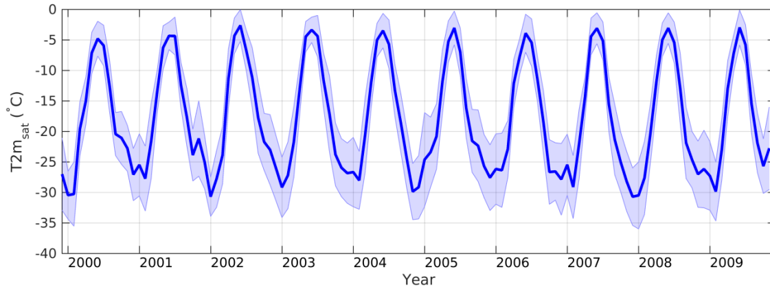
10 Figure 14: Monthly mean T2m_{sat} for the Greenland Ice Sheet. The shading represents the variability.
