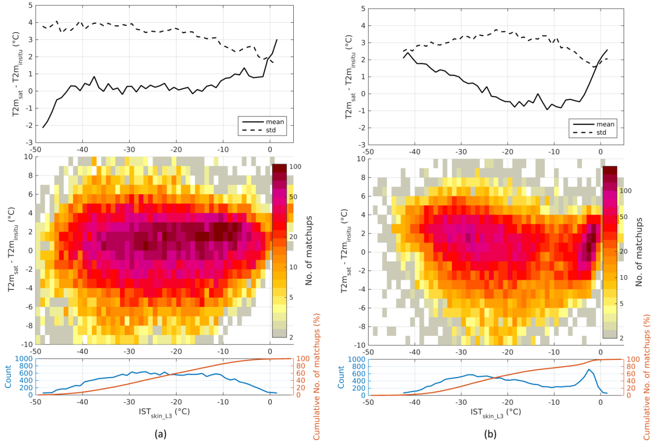
Figure 10: Estimated T2m minus observed T2m (bin size of 1°C) as a function of binned (bin size of 1°C) satellite IST skin_L3 for (a) land ice and (b) sea ice. The dashed lines are standard deviations while the solid lines are bias in the upper figure. The surface plots in the middle figures show the number of matchups in each bin while the bottom plots show the number of matchups (blue) and the cumulative percentage of matchups (red) in each IST skin_L3 bin.
