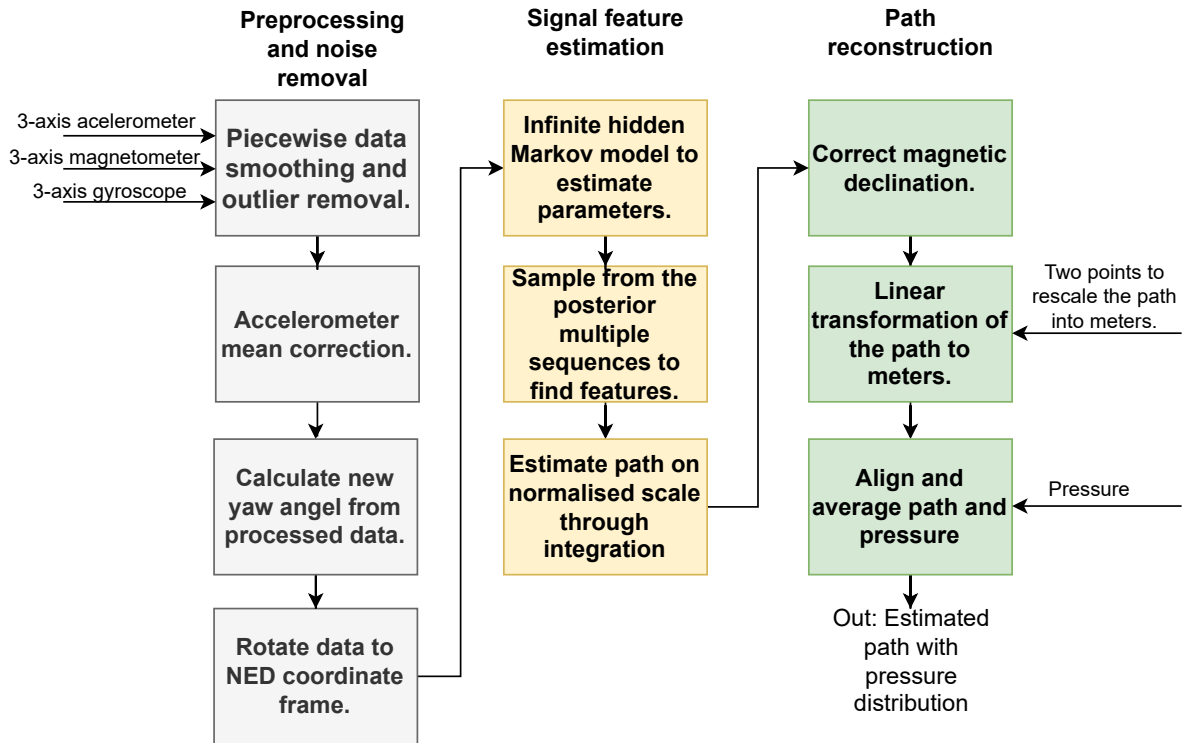
Figure 4. Workflow diagram of the processing sequence. The model applies an infinite hidden Markov model (iHMM, see Beal et al. (2002)) on the IMU data to detect signal features. NED stands for north-east-down.
