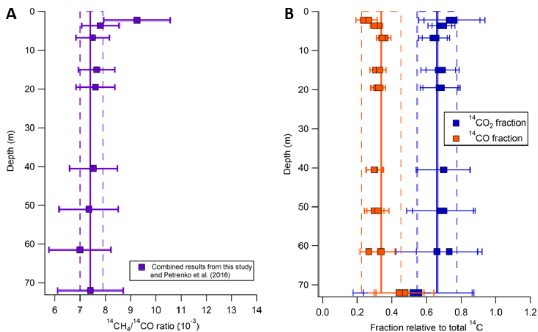
Fig. 4. (A) ^{14}\text{CH}_4/^{14}\text{CO} ratio. (B) ^{14}\text{CO}_2/\text{total } ^{14}\text{C} fraction and ^{14}\text{CO}/\text{total } ^{14}\text{C} fraction. The solid lines represent the mean and the dashed lines represent 2 standard deviations of the ^{14}\text{CH}_4/^{14}\text{CO} ratio, ^{14}\text{CO}_2 and ^{14}\text{CO} fractions for samples deeper than 6.85 m where production by muons dominates. The ratios for rejected samples (Section 4.1, Supplementary Materials Section 2) are not shown. All error bars shown in this figure are 95% CI.
