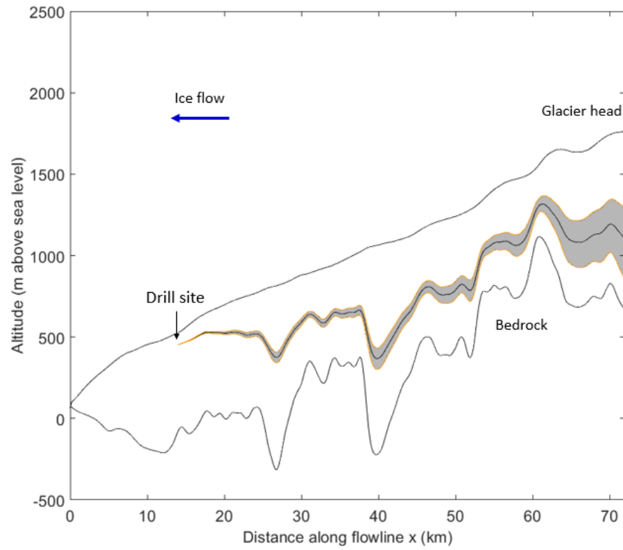
Fig. 5. Example of ice parcel back-trajectory and associated uncertainties. For the Monte-Carlo estimate of uncertainties (Section 5.4.2), for each given sample depth (72 m in this figure), 10,000 back trajectories are generated. Each back trajectory corresponds to a different ablation rate scenario (the ablation rates are perturbed within their experimental measurement uncertainties to generate the scenarios). The shaded region represents the 68% CI uncertainty envelope of the flow trajectory.
